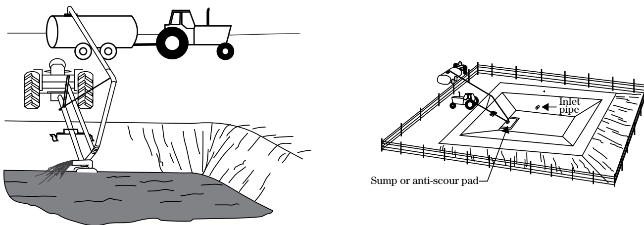
Figure 10-20 Waste storage ponds
