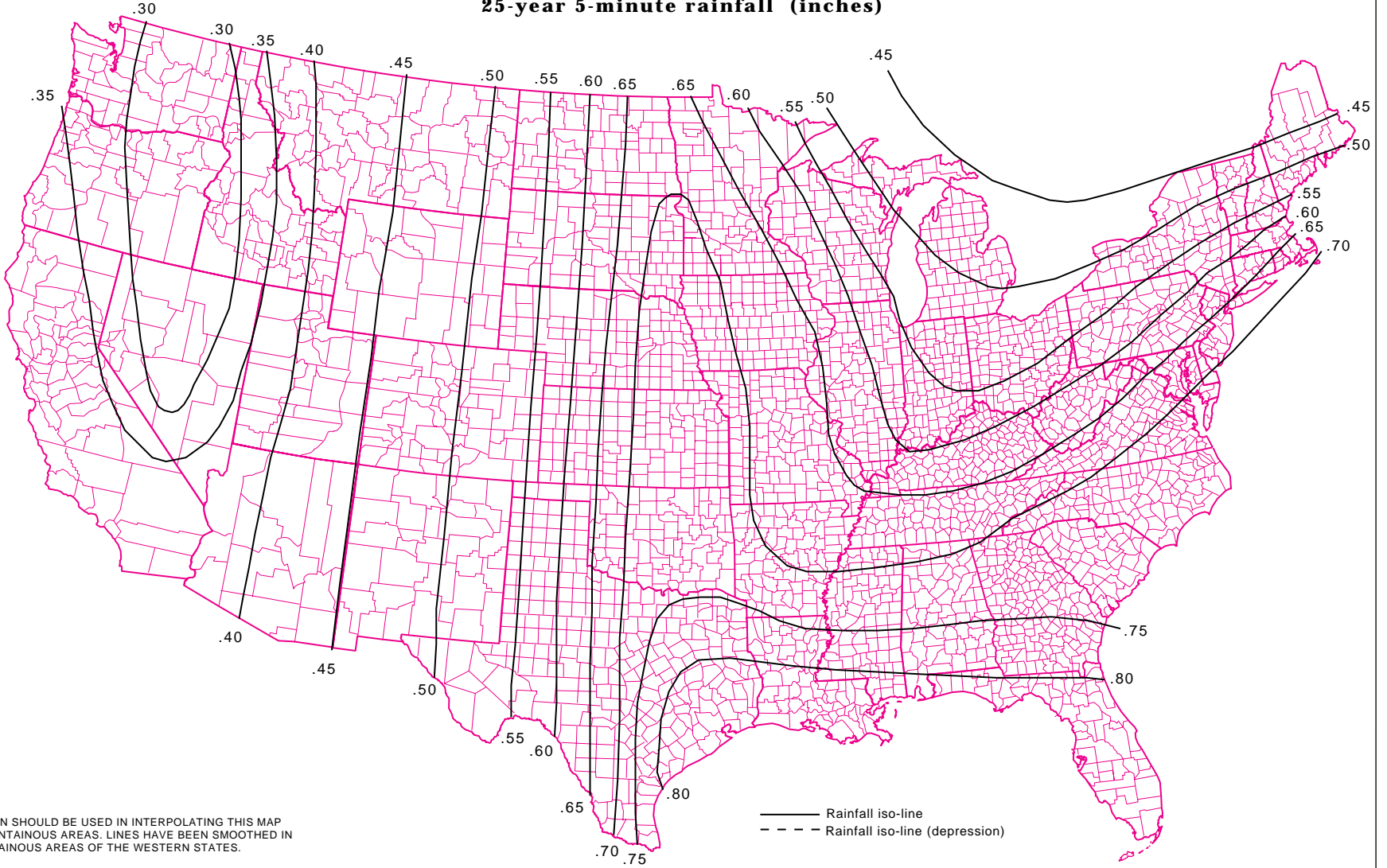
Figure 10B-4 25-year 5-minute rainfall (inches)
