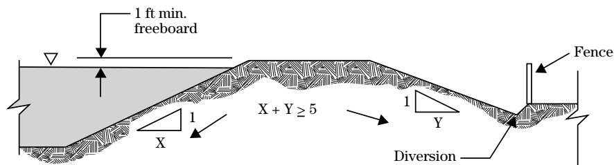
Cross-section earth embankment
