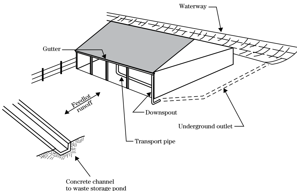
Figure 10–1 Roof gutter and downspout
