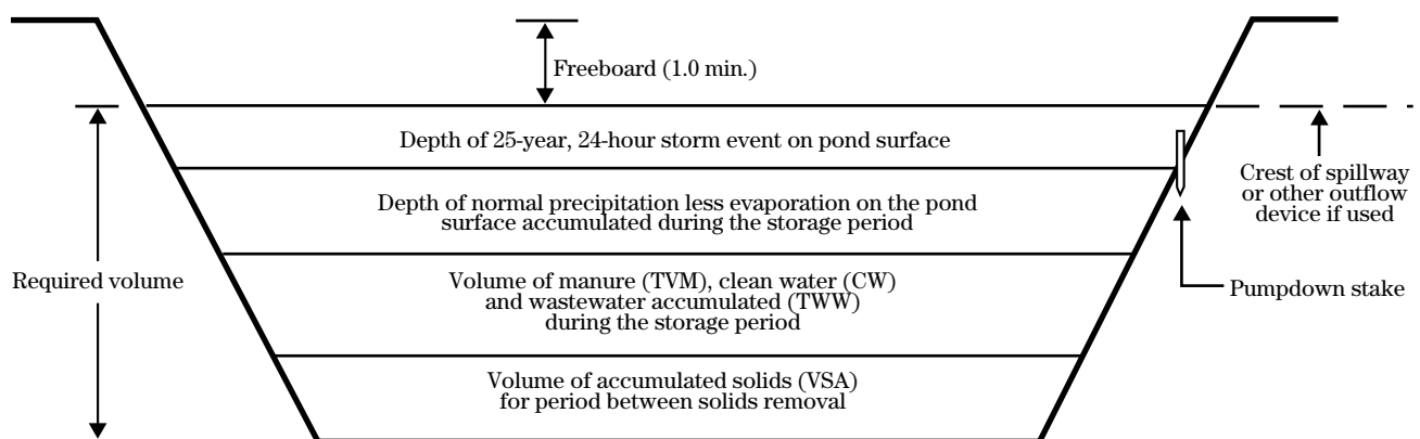
Figure 10-18 Cross section of waste storage pond without a watershed
