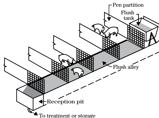
Figure 10-5 Swine flush alley
