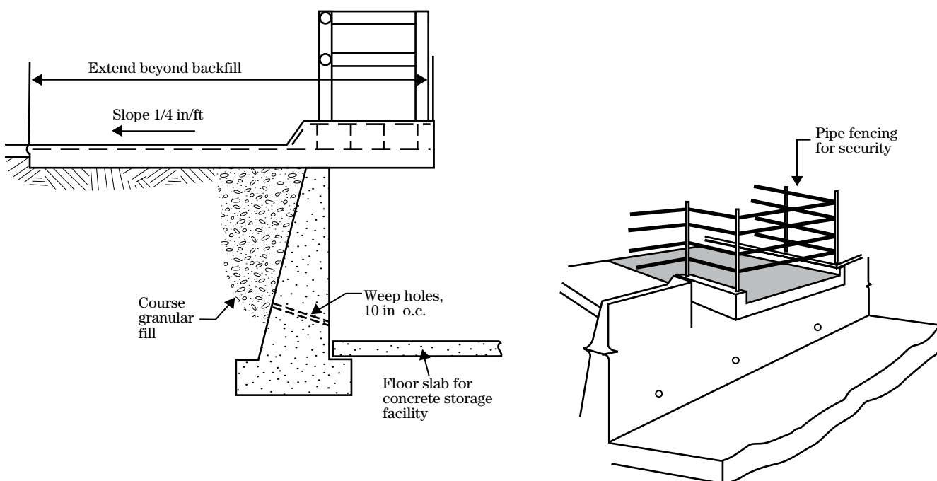
Figure 10-14 Push-off ramp
