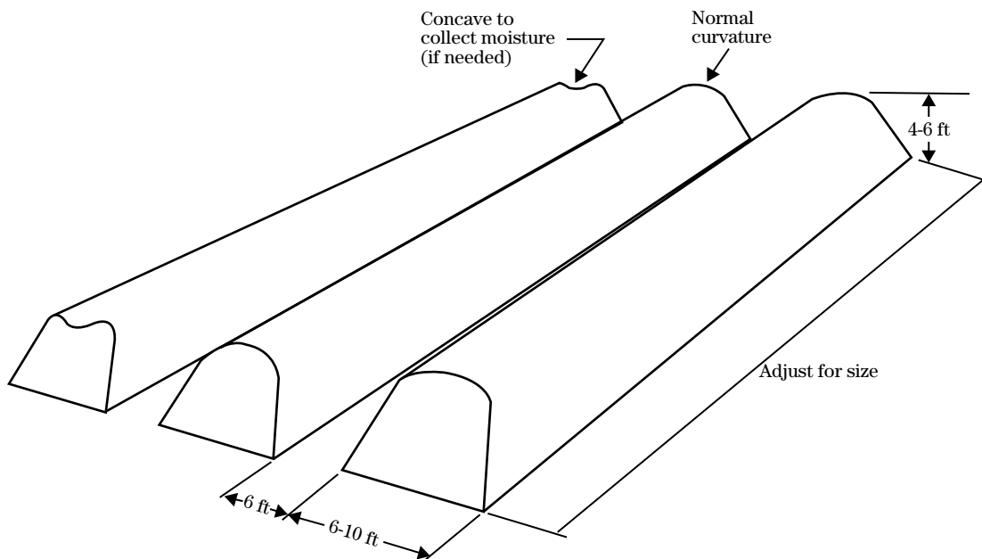
Figure 10–35 Windrow schematic
