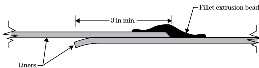
Figure 10E-15 Extrusion weld
