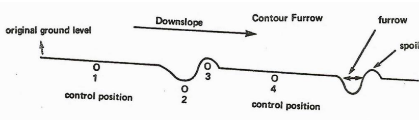
Figure D-7. Cross section of furrowed hillslope showing relative position of sampling points (Hawkins et al., 1977).
