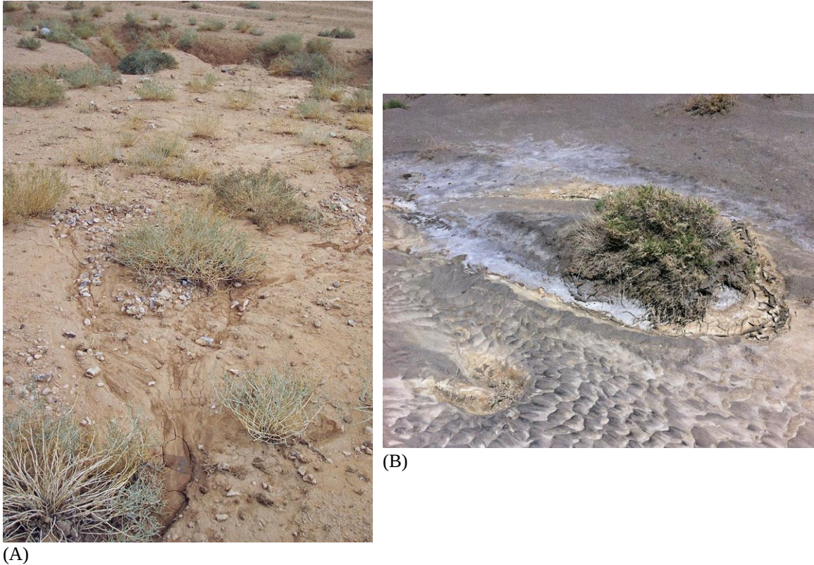
Figure C-9. (A) Vegetation islands redirecting concentrated flow around, resulting in deposition on the down slope side of the hillslope. (B) Greasewood coppice dunes illustrating interconnected bare spaces and linked concentrated flow paths that readily transport salt in surface runoff or are vulnerable to wind transport of soils and salt.
