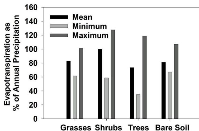
Figure A-7. Estimated averages and ranges (as maximum and minimum) of annual evapotranspiration as percentage of annual precipitation for various rangeland plant types as reported in literature (Brandes and Wilcox, 2000; Carlson and Thurow, 1996; Carlson et al., 1990; Flerchinger and Cooley, 2000; Flerchinger et al., 1998; Joffre and Rambal, 1993; Weltz and Blackburn, 1995). (Caption and figure from Pierson and Williams, 2016.)
