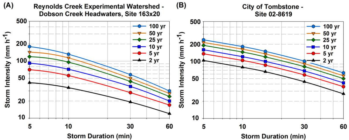
Figure A-4. Intensity-duration-frequency graphs for (A) climate station 163x20 at 2,170 m elevation in the snowfall-dominated Reynolds Creek Experimental Watershed, Idaho, 1963 to 1998 (Hanson and Pierson, 2001); (B) climate station 02-8619 at 1,400 m elevation, Tombstone, Arizona, near the summer monsoon rainfall-dominated Walnut Gulch Experimental Watershed, 1893 to 2000 (Bonnin et al., 2006). (Caption and figure from Pierson and Williams, 2016.)
