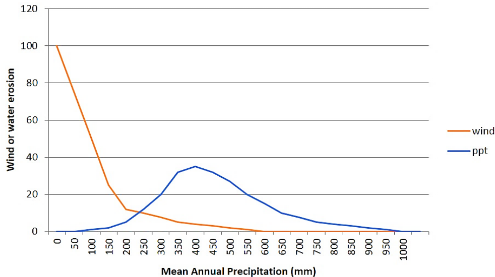
Figure C-2. Conceptual diagram of wind and water erosion with mean annual precipitation for naturally vegetated arid and semi-arid range lands (Modified from Marshall 1973).
