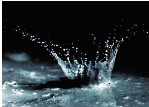
(A) Raindrop splash erosion.
