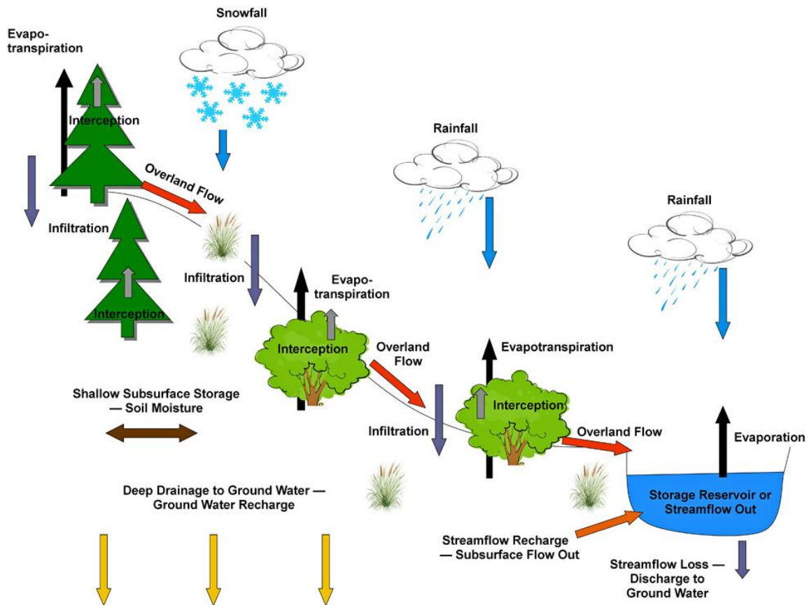
Figure A-2. Illustration of the generalized hydrologic cycle for a hillslope showing directional inflows (rainfall, snowfall, infiltration) and outflows (evapotranspiration, losses to interception, overland flow, deep drainage, streamflow, and subsurface flow out). (Caption and figure from Pierson and Williams, 2016.)
