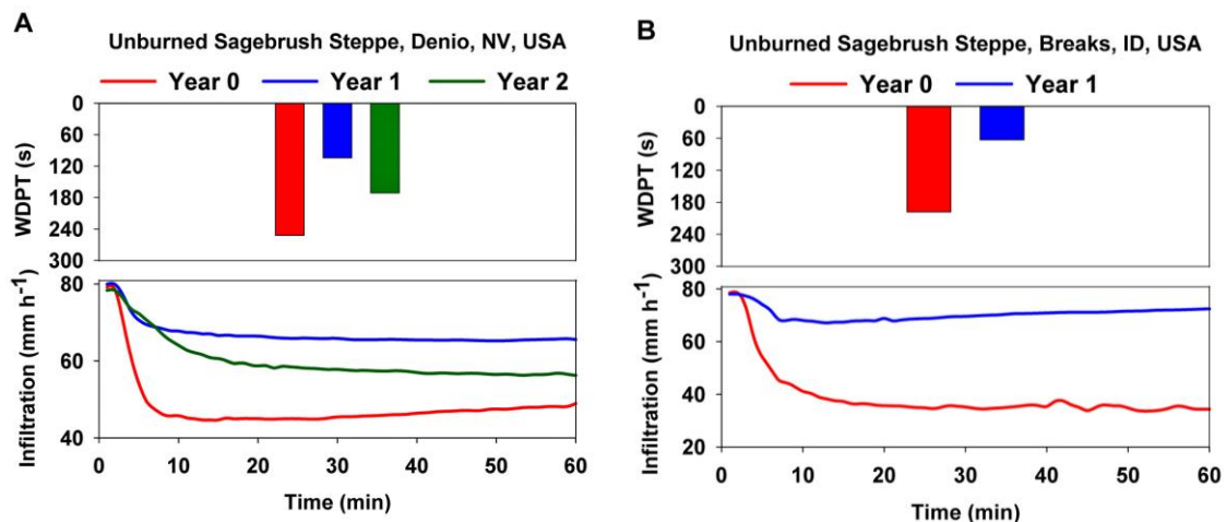
Figure B-7. Temporal variability of soil water repellency effects (measured by using water drop penetration time, WDPT) on infiltration of artificial rainfall into unburned, coarse-textured soils at two sagebrush sites: (A) Denio Fire (wildfire), Pine Mountain Range, Nevada (Pierson et al., 2008b); and (B) Breaks Prescribed Fire, Reynolds Creek Experimental Watershed, Idaho (Pierson et al., 2009). WDPT is an indicator of strength of soil water repellency as follows: <5 s wettable, 5 to 60 s slightly repellent, 60 to 600 s strongly repellent (Bisdorn et al., 1993). (Caption and figure from Pierson and Williams, 2016.)
