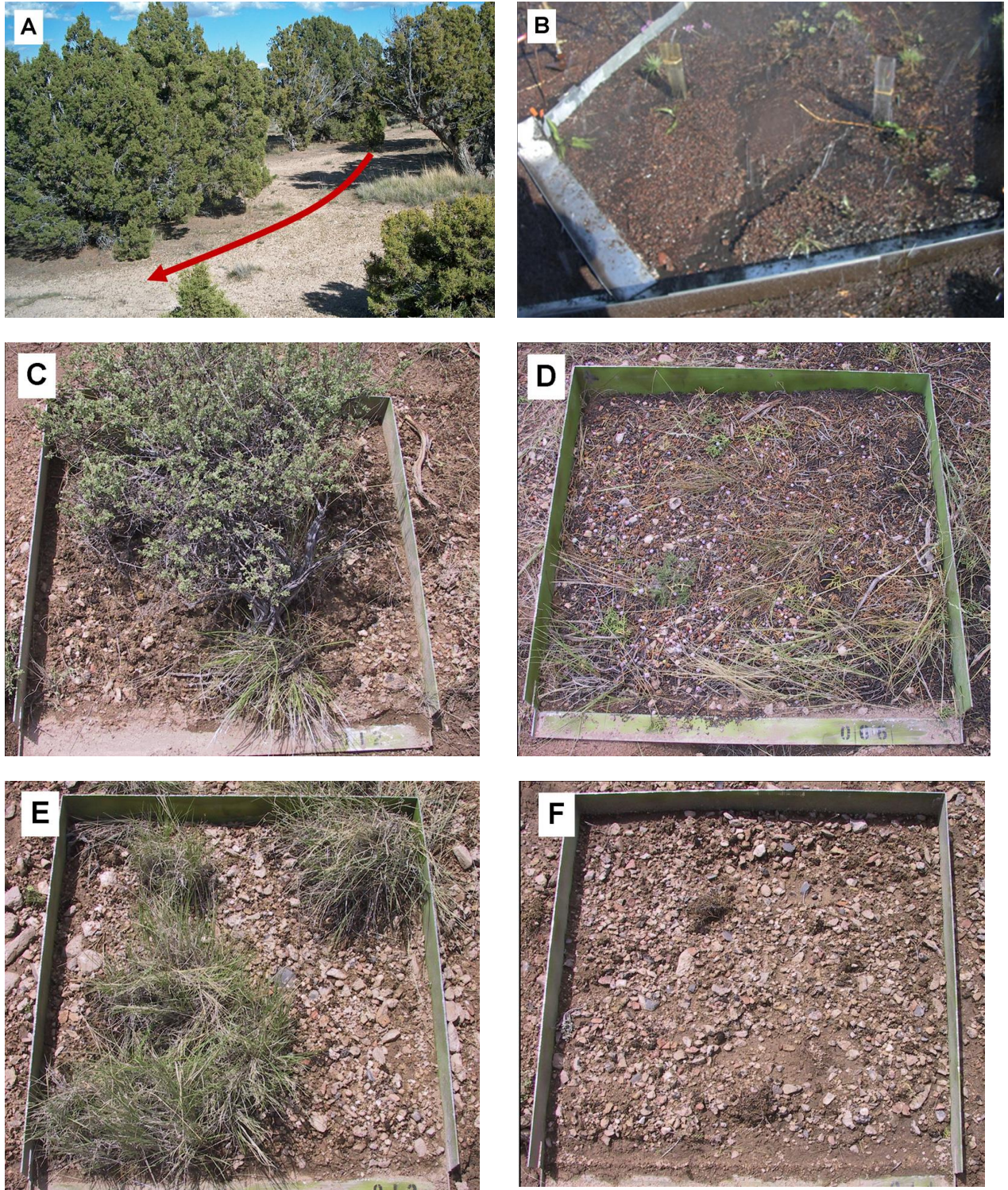
Figure C-5. Photographs from a Utah Juniper woodland site in Utah, showing (A) general direction for overland flow over contiguous bare interspace, (B) interspace concentrated flow path during artificial rainfall simulation, (C) hydrologically stable shrub, (D, E, F) and vegetated and bare interspaces (photos: USDA Agricultural Research Service, Northwest Watershed Research Center). (Caption and figure from Pierson and Williams, 2016.)
