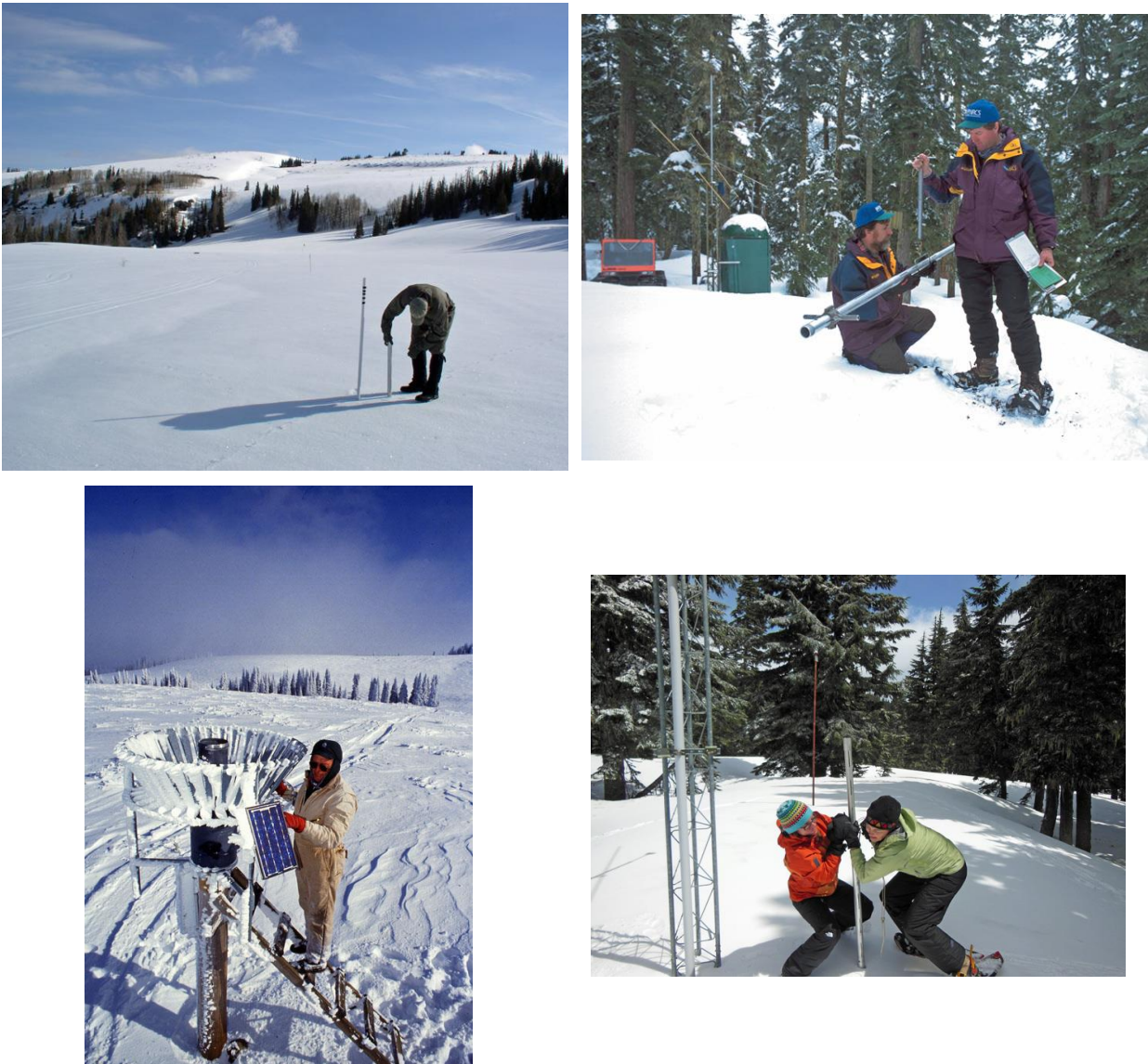
Figure D-13. Measuring snow fall and soil water equivalent at the USDA Agricultural Research Service Reynolds Creek Experimental Watershed near Boise, Idaho.
