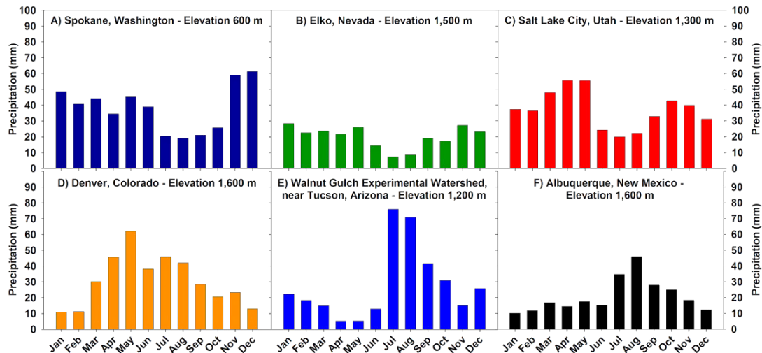
Figure A-6. Average monthly precipitation for western U.S. urban centers immediately adjacent to rangelands (PRISM, 2011). Panels A–C are indicative of annual precipitation in the Inland Northwest. Panel D is indicative of annual precipitation trends on central U.S. rangelands. Panels E–F demonstrate the influence of the monsoonal season (July–August) on the rainfall in the desert Southwest. (Caption and figure from Pierson and Williams, 2016.)
