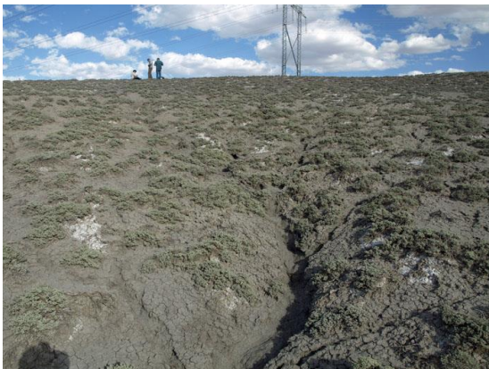
Figure B-5. Gully erosion on an unprotected soil in central Utah.
