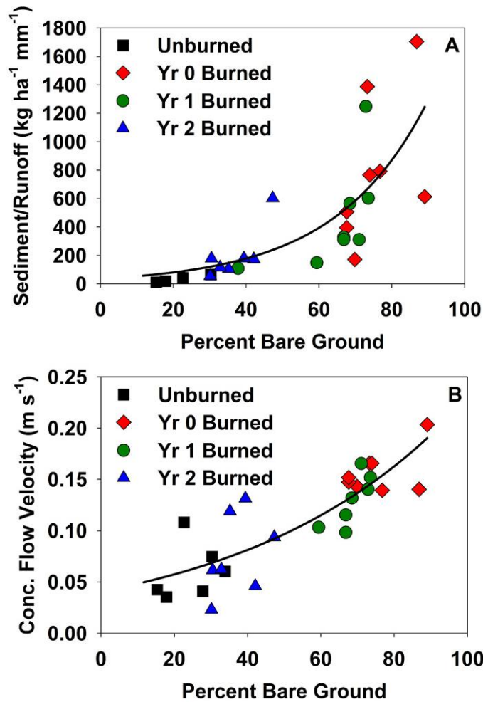
Figure C-4. Sediment per unit of runoff (A) and concentrated flow velocity (B) versus percent bare ground measured on rainfall simulation plots (32.5 m 2 , 85 mm h -1 rainfall intensity) and concentrated flow experiments (12 L min -1 flow release) on unburned and burned shrublands. Data from Pierson et al. (2009). (Caption and figure from Williams et al., 2014; Nouwakpo et al., 2016.)
