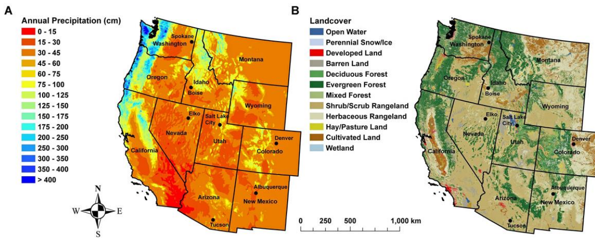
Figure A-5. (A) Annual precipitation (PRISM, 2011) and (B) landcover (U.S. Geological Survey 2011) for the western United States. (Caption and figure from Pierson and Williams, 2016.)
