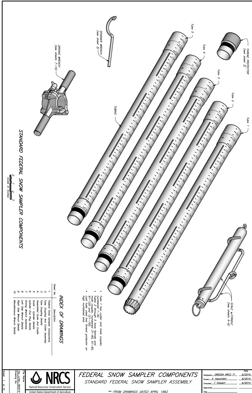
Figure 8G-2 Federal snow sampler, 1 of 10
