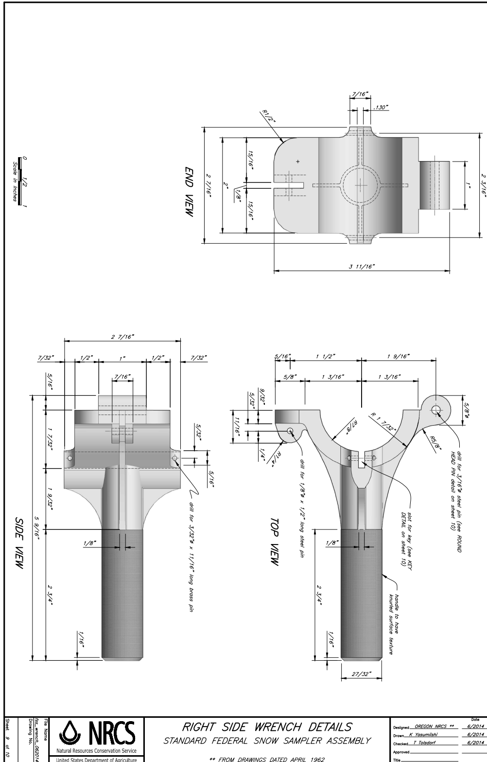
Figure 8G-2 Federal snow sampler, 9 of 10—continued
