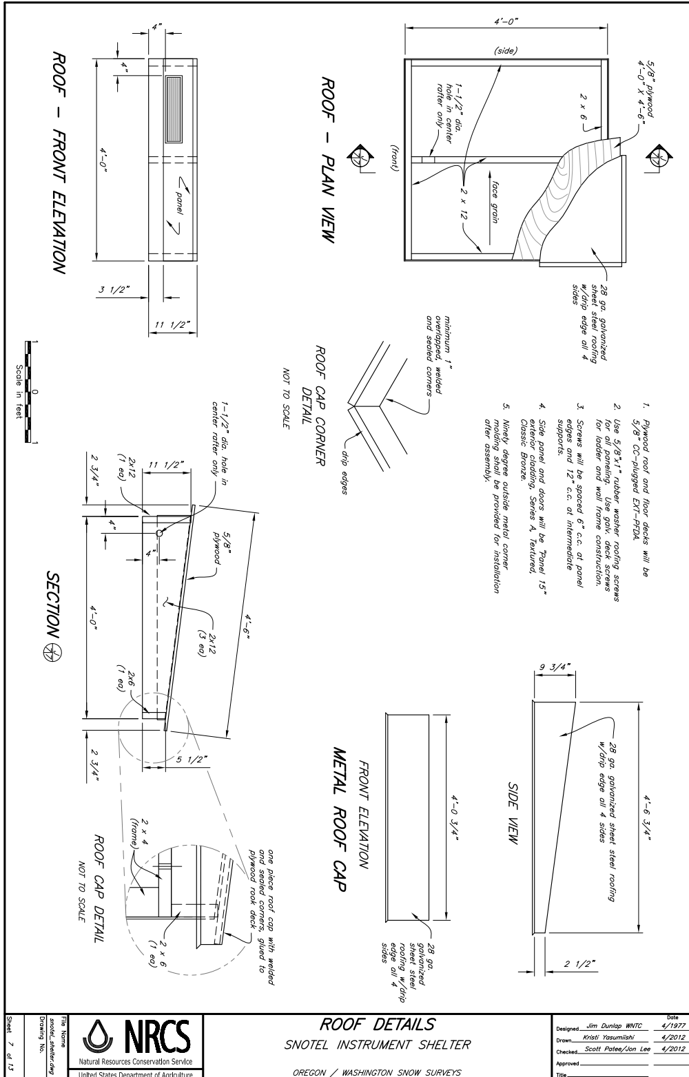
Figure 8G-4 SNOTEL shelter, 7 of 13—continued
