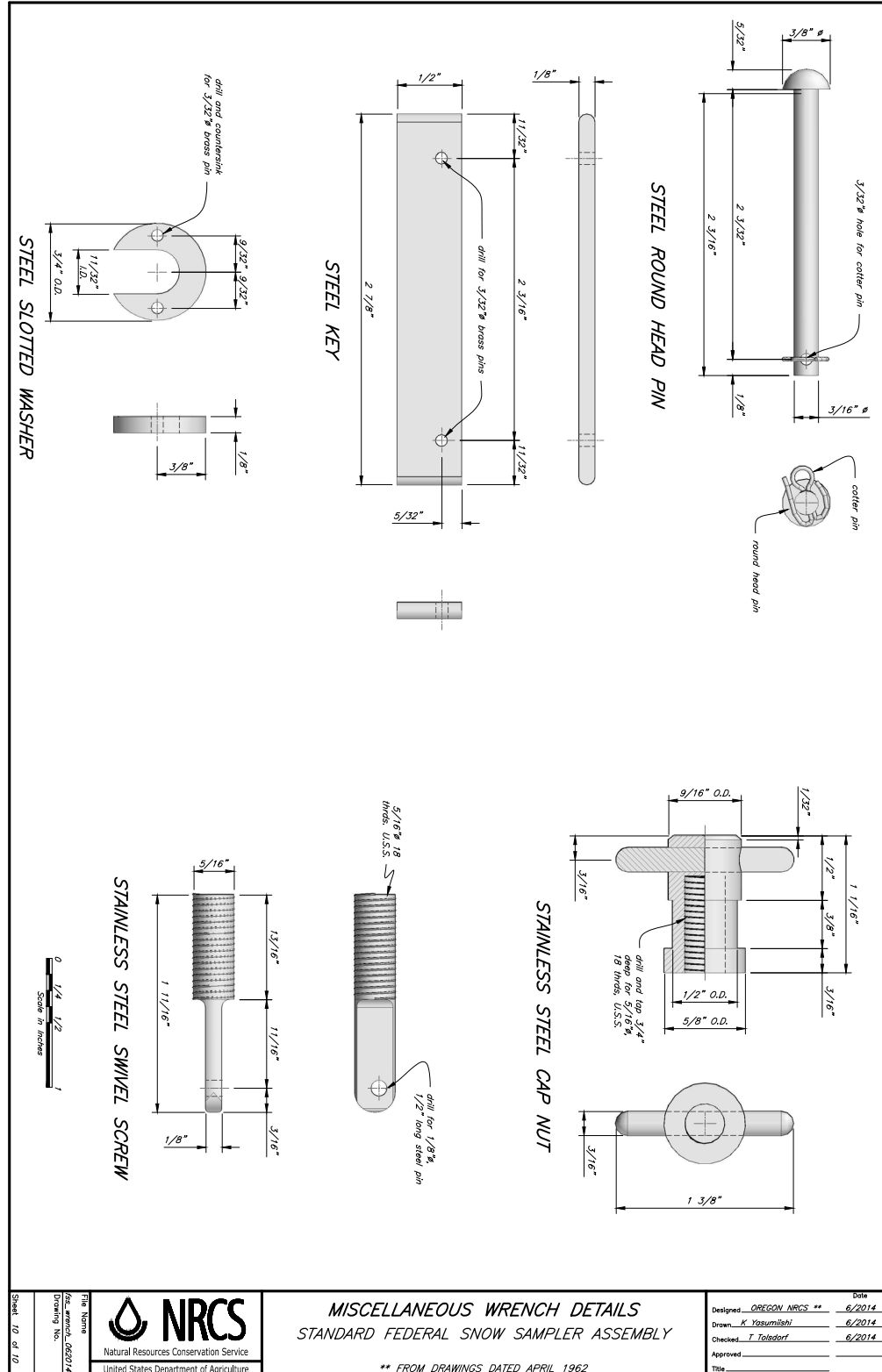
Figure 8G-2 Federal snow sampler, 10 of 10—continued
