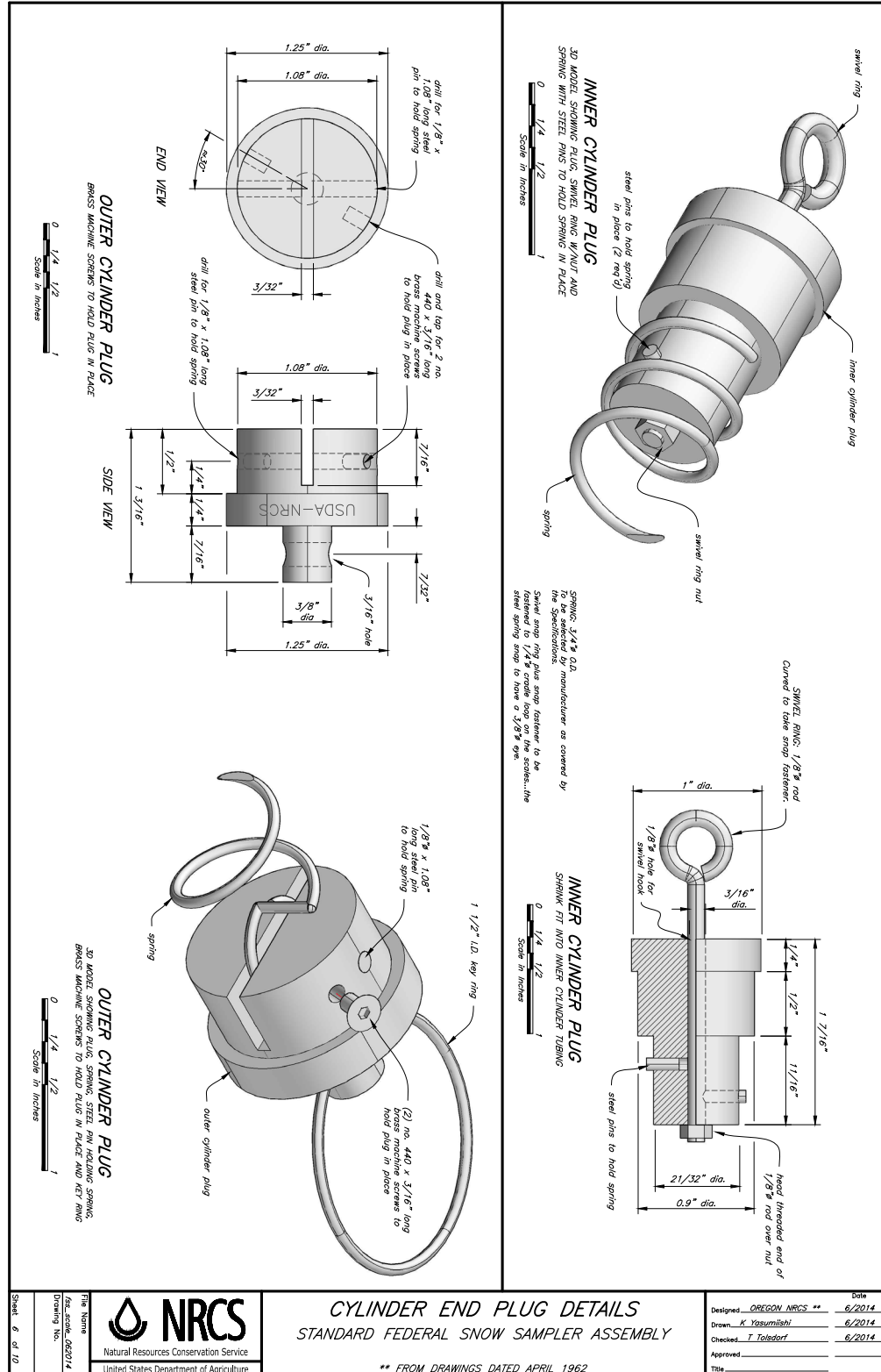
Figure 8G-2 Federal snow sampler, 6 of 10—continued
