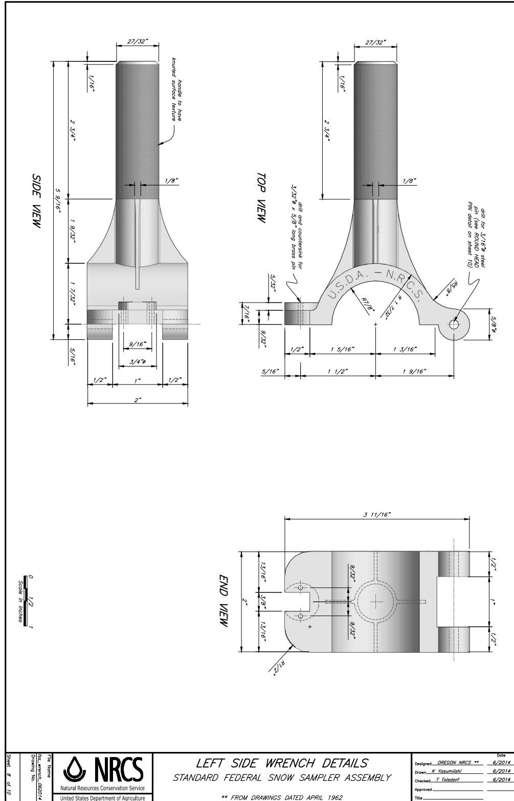
Figure 8G-2 Federal snow sampler, 8 of 10—continued
