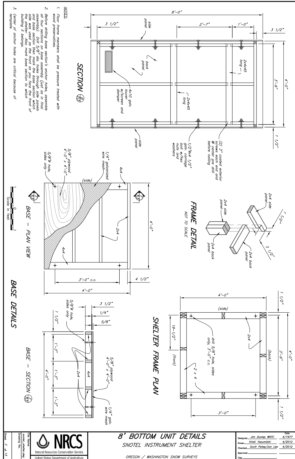
Figure 8G-4 SNOTEL shelter, 3 of 13—continued
