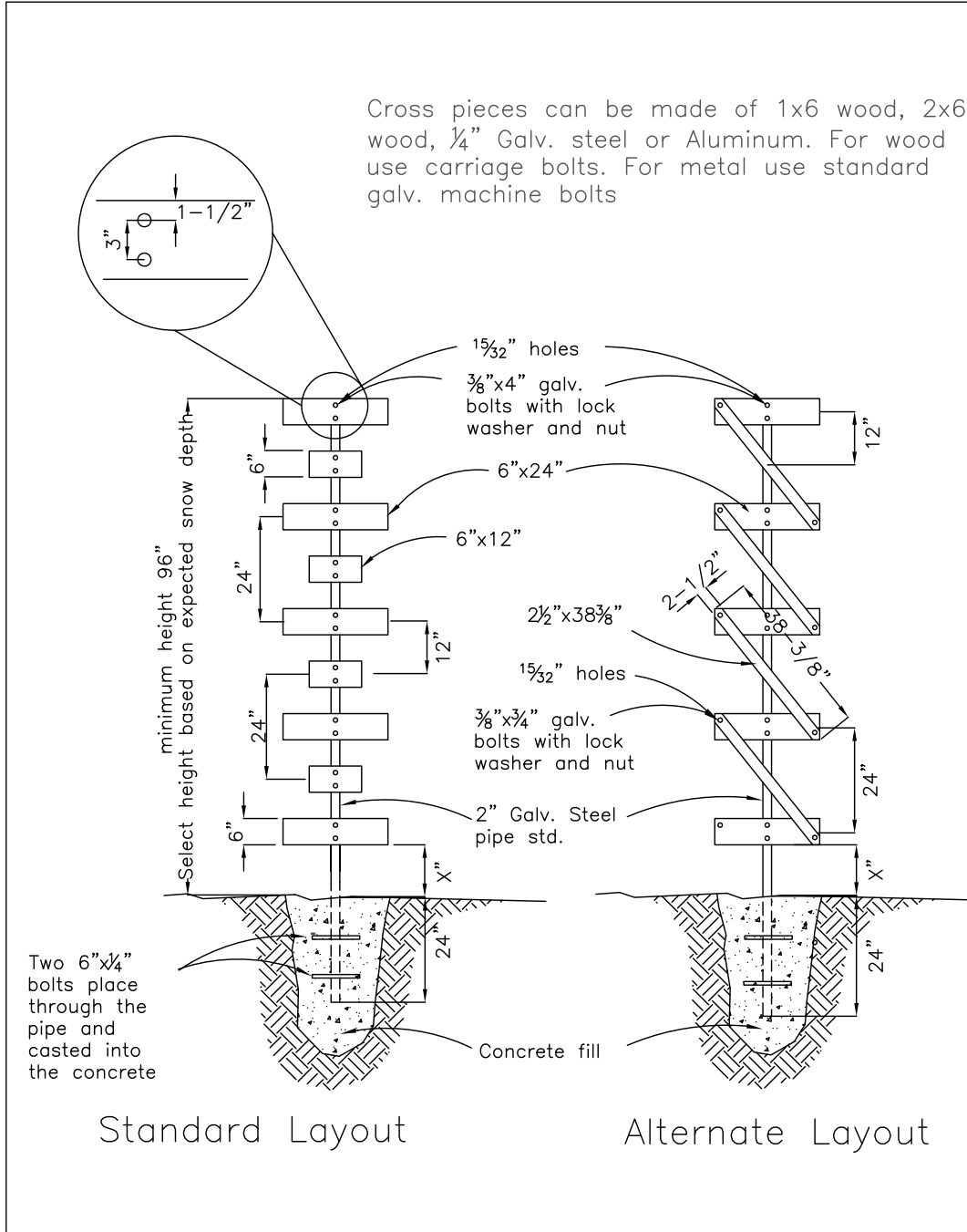
Figure 8G-1 Standard drawings
