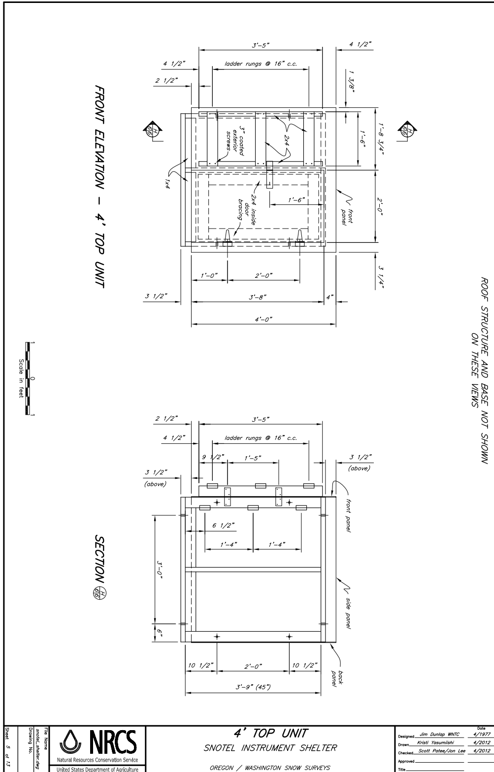
Figure 8G-4 SNOTEL shelter, 5 of 13—continued
