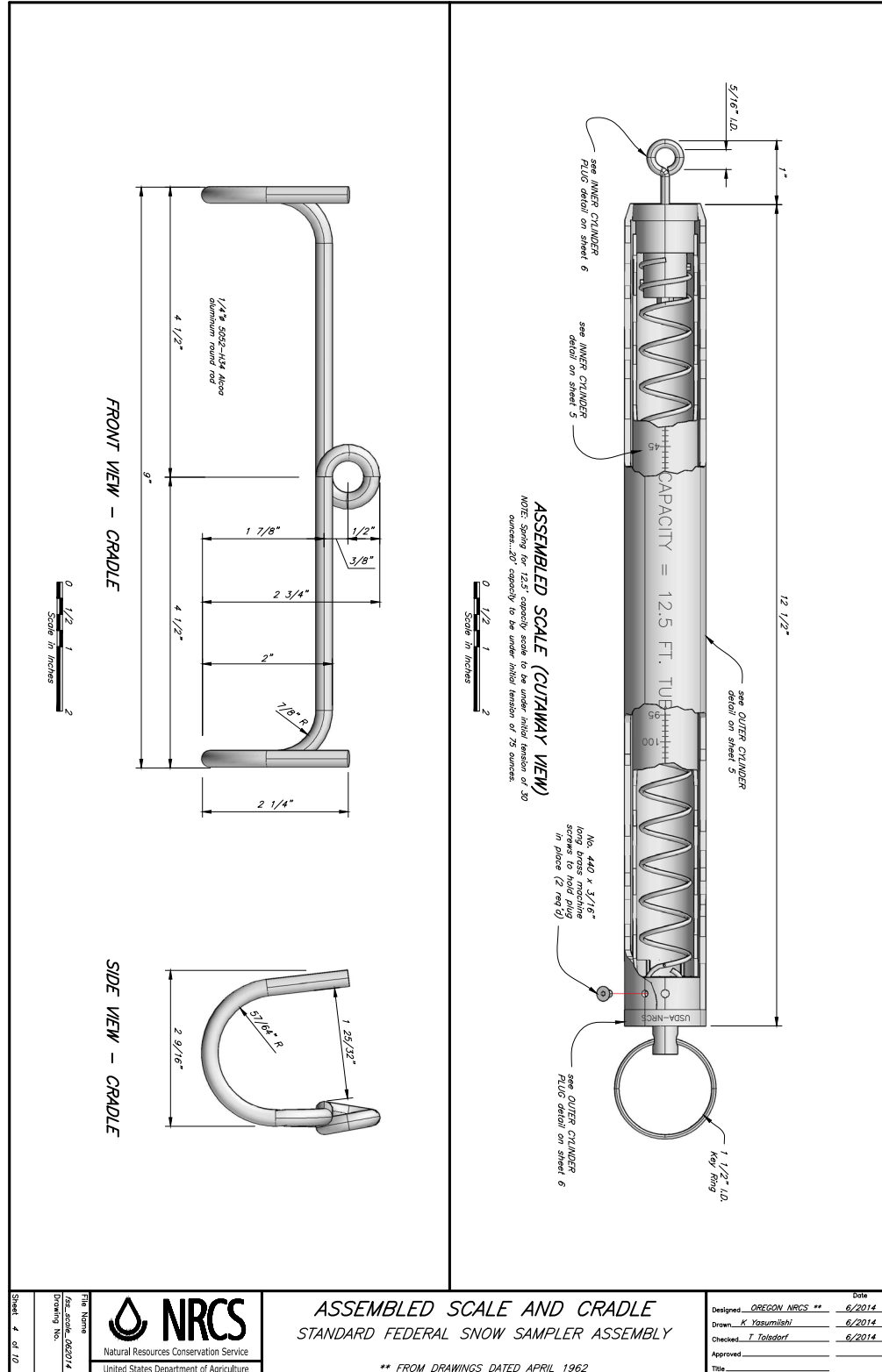
Figure 8G-2 Federal snow sampler, 4 of 10—continued
