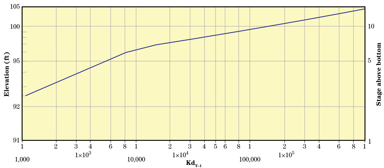
Figure 14–10 Conveyance values, section T-1, example 14–6
