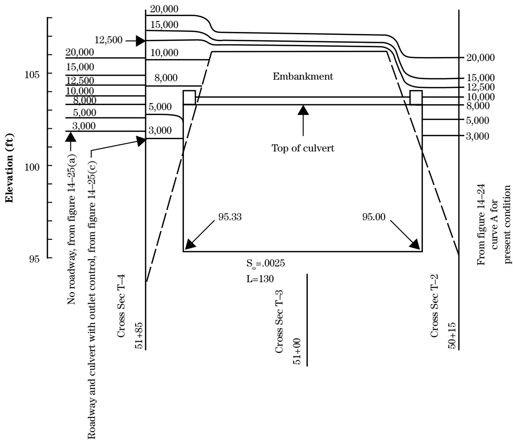
(b) Profile through culvert
