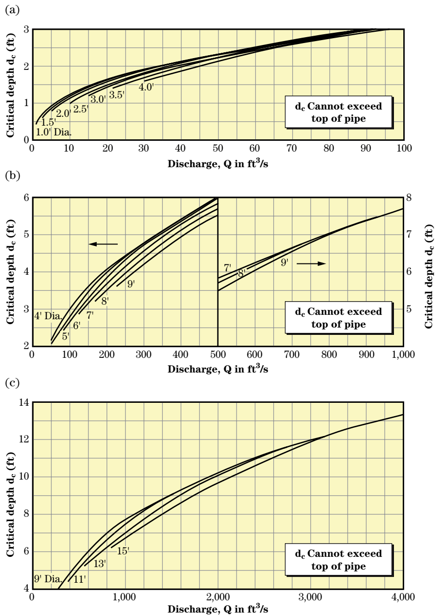
Exhibit 14-17 Critical depth—circular pipe
