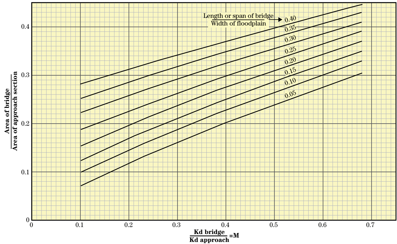
Exhibit 14-3 Estimate of M for use in BPR equation
