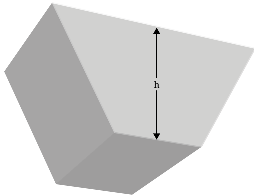
Figure 5-8 Prismatoid
