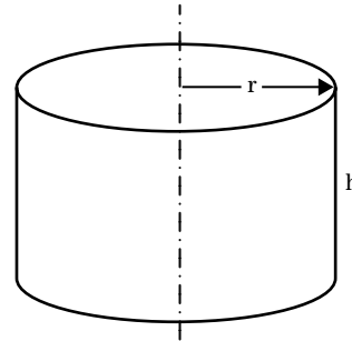
Figure 5-9 Cylinder
