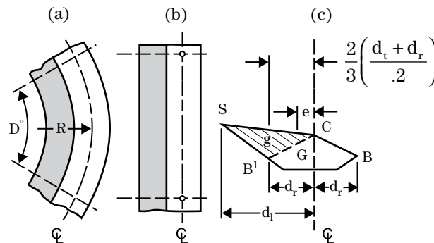
Figure 5-13 (a) Representation of volume corrected for curvature (b) Representation of volume not corrected for curvature (c) Asymmetrical section
