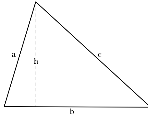
Figure 5-5 General triangle
