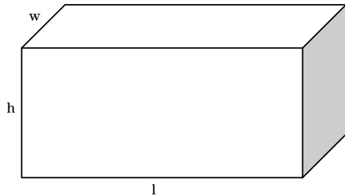
Figure 5-7 Rectangular prism
