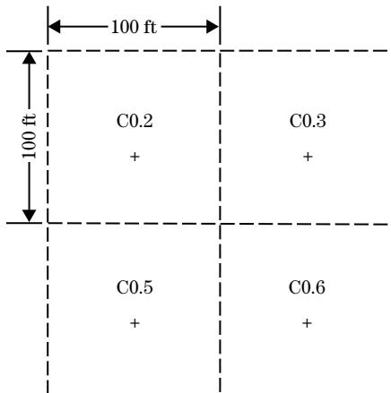
Figure 5–14 Area to be excavated represented by four points and the depth of cut at each point
