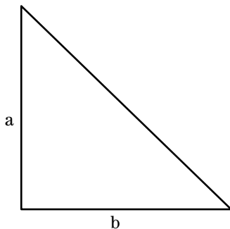
Figure 5-4 Right triangle
