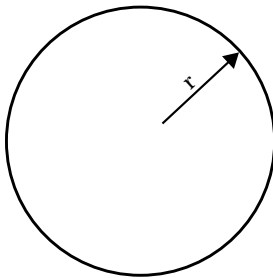
Figure 5-3 Circle
