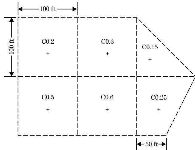
Figure 5–15 Area to be excavated represented by six points and the depth of cut at each point
