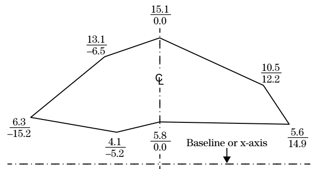
Figure 5-6 Irregular shape defined by rectangular coordinates in feet
