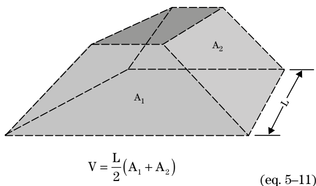
Figure 5-11 Volume between two parallel ends
