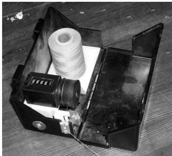
Figure 1-33: String Box or Hip Chain
