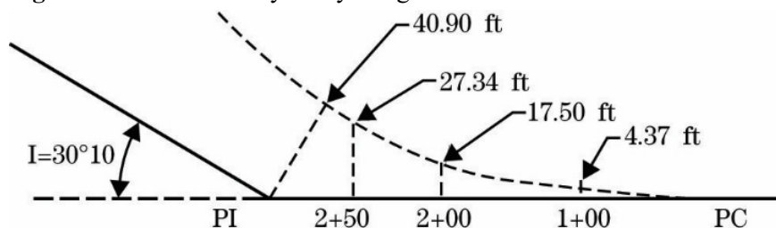
Figure 1-102: Curve Layout by Tangent Offsets
