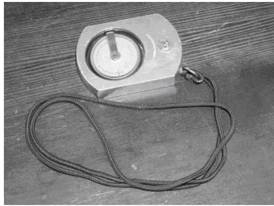
Figure 1-44: Clinometer
