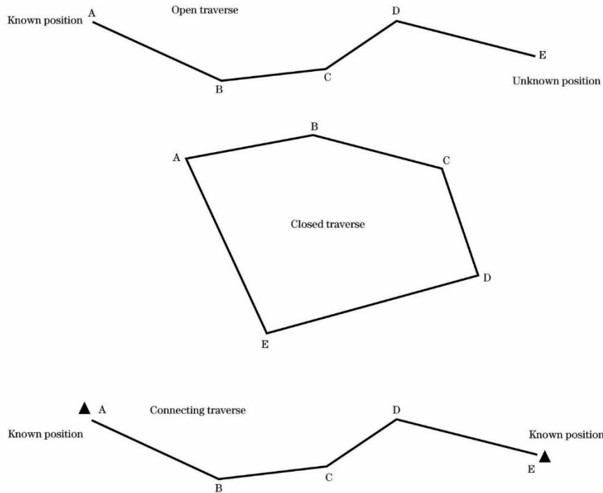
Figure 1-12: Open Traverse
