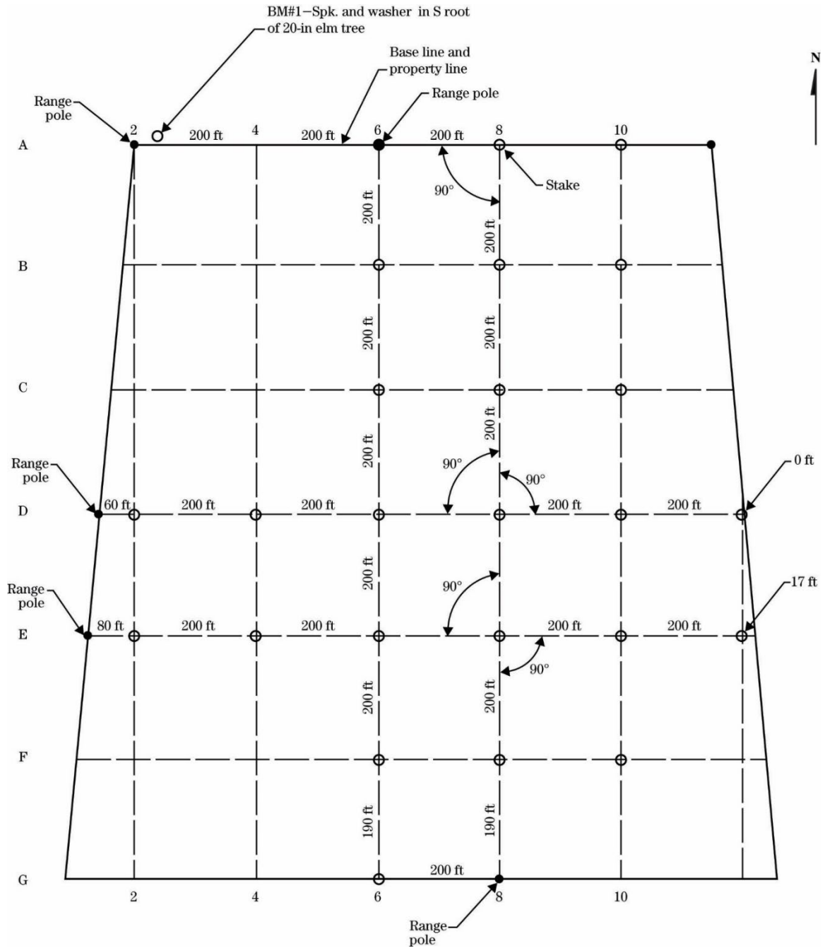
Figure 1-64: Method of Topographic Survey by Gridding
