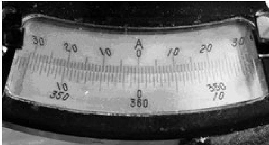
Figure 1-56: One-minute Vernier Set at 0 Degrees
