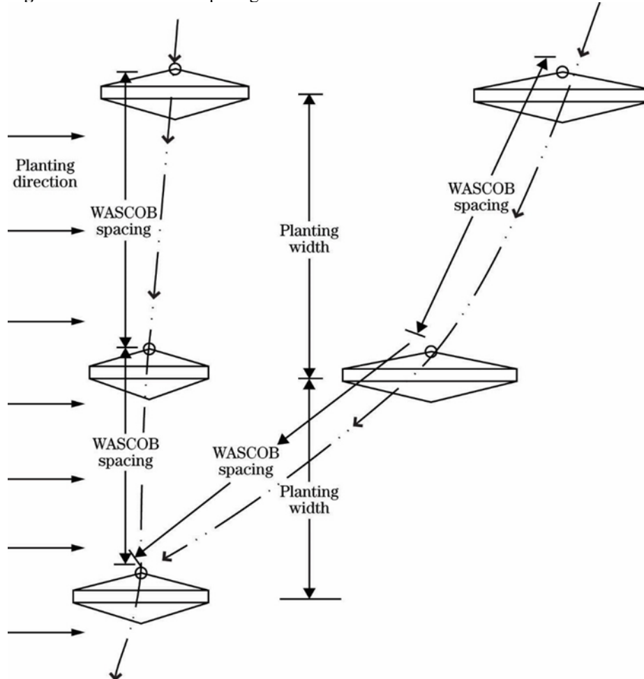
Figure 8-12: WASCOB Spacing
