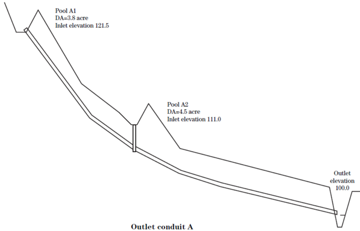
Figure 8A-2: Pressure Flow System
