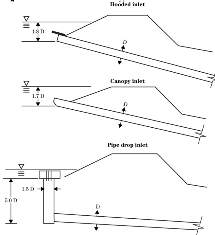
Figure 8-52: Pressure Flow Inlet Types
