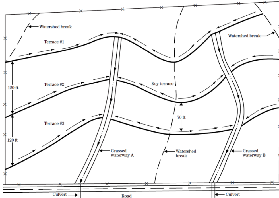
Figure 8-28: Typical Gradient Alignment Layout
