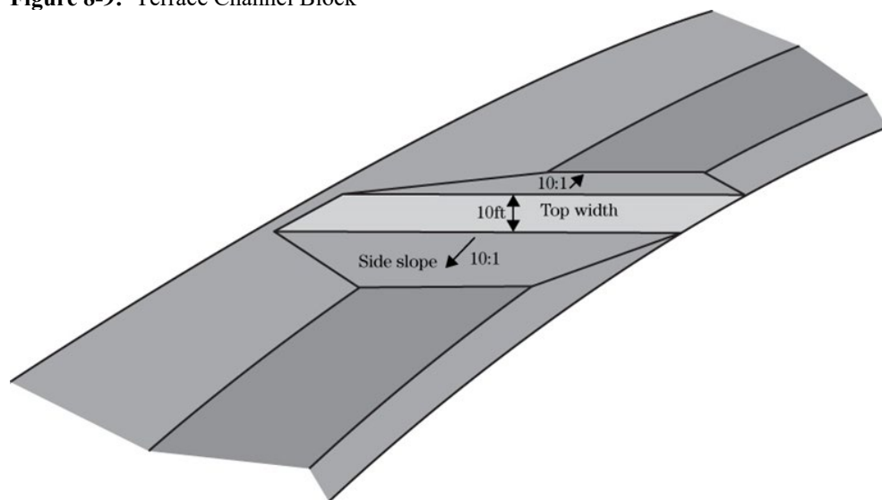
Figure 8-9: Terrace Channel Block
