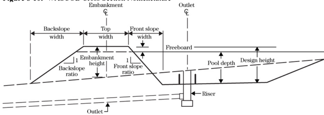
Figure 8-10: WASCOB Cross Section Nomenclature
