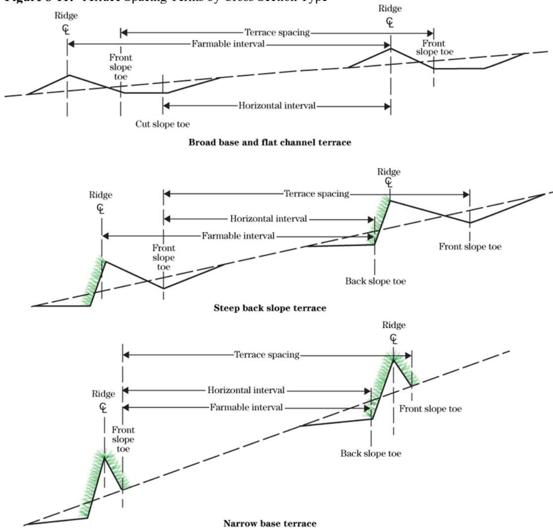
Figure 8-11: Terrace Spacing Terms by Cross Section Type
