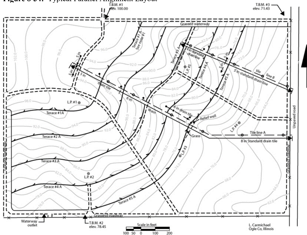
Figure 8-34: Typical Parallel Alignment Layout
