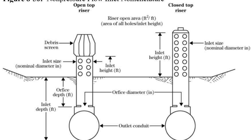
Figure 8-50: Nonpressure Flow Inlet Nomenclature
