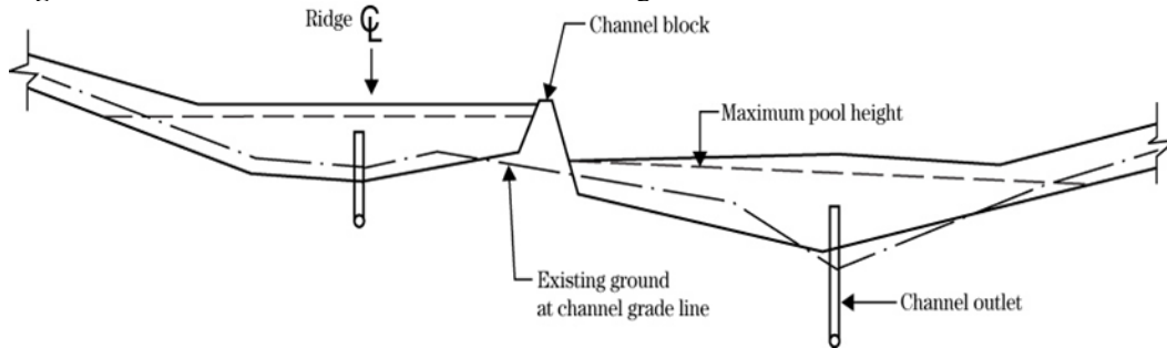
Figure 8-31: Use of Channel Blocks for Parallel Alignment
