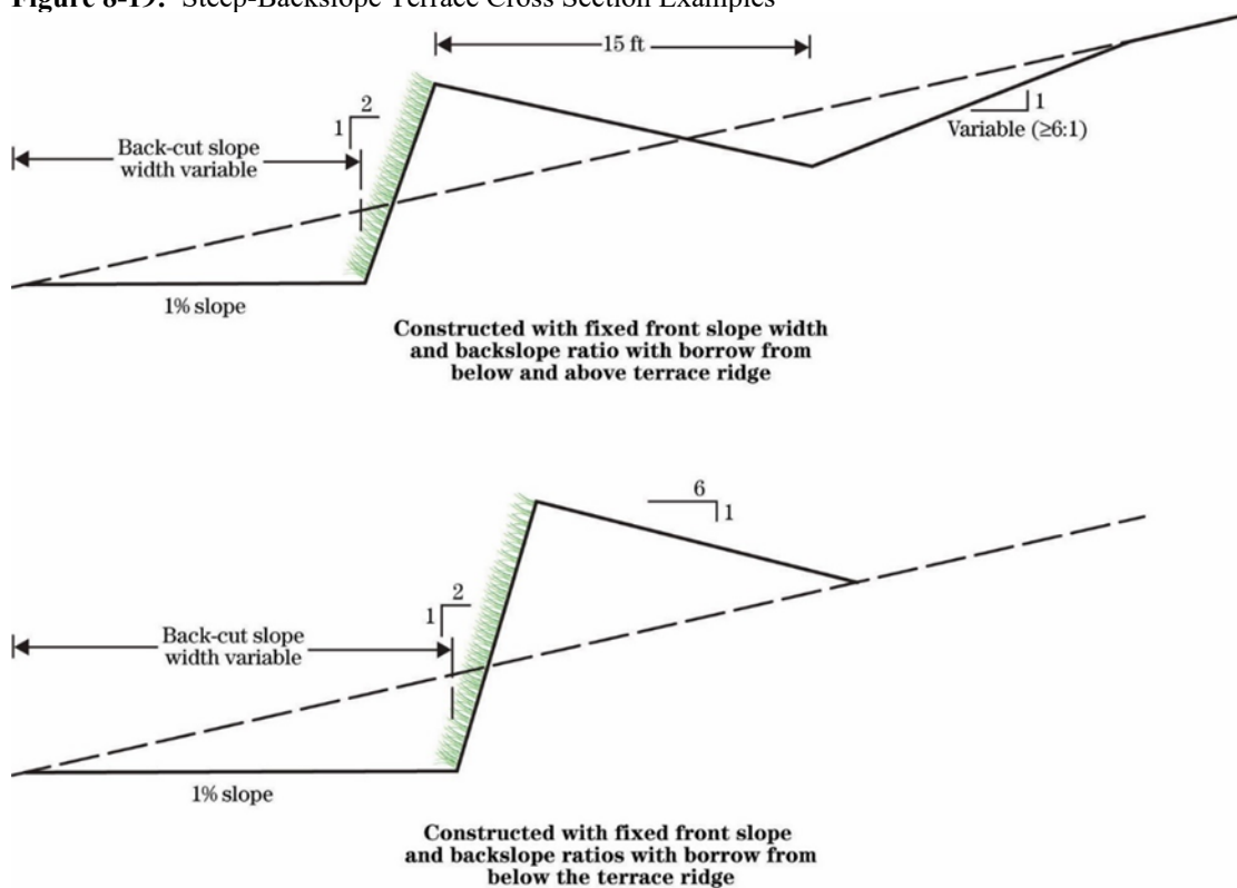
Figure 8-19: Steep-Backslope Terrace Cross Section Examples
