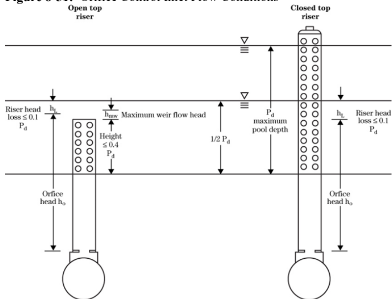
Figure 8-51: Orifice Control Inlet Flow Conditions
