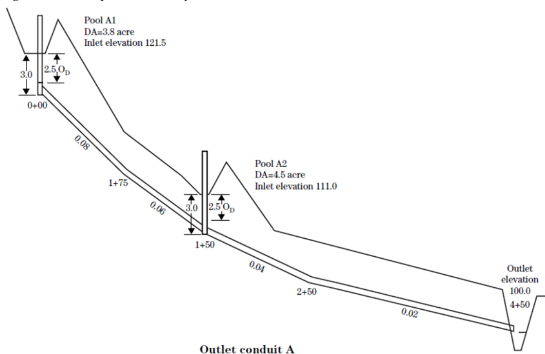
Figure 8A-1: Nonpressure Flow System
