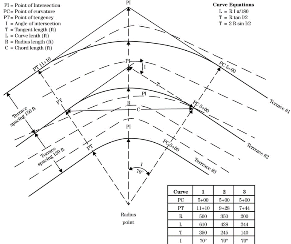
Figure 8-30: Concentric Circular Curves
