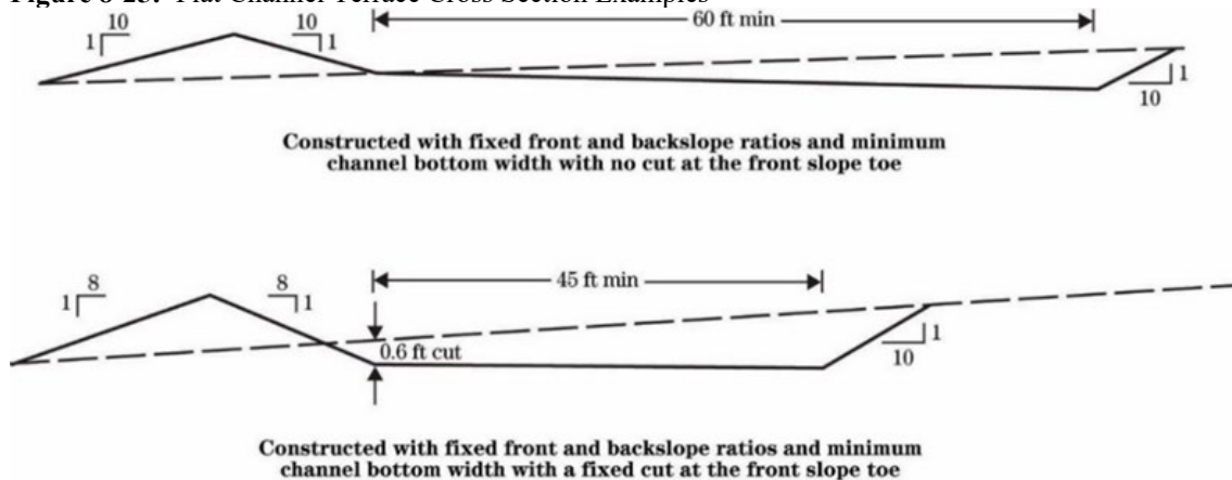
Figure 8-25: Flat Channel Terrace Cross Section Examples
