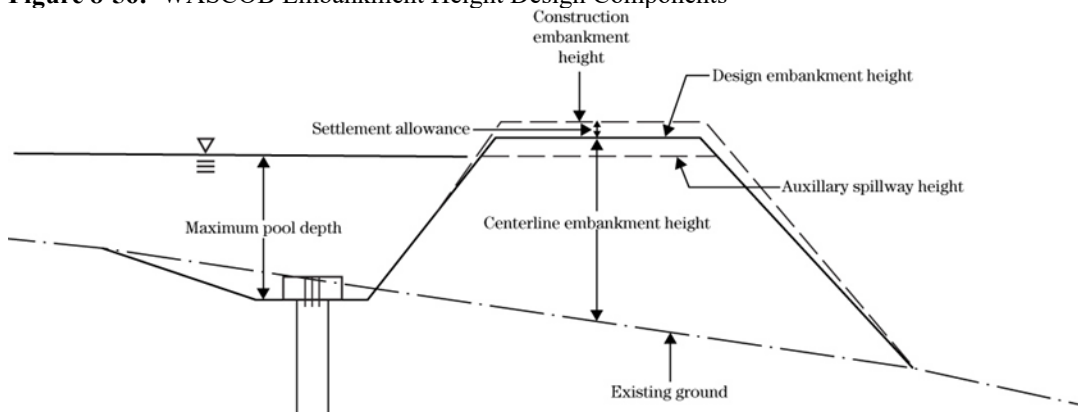
Figure 8-56: WASCOB Embankment Height Design Components
