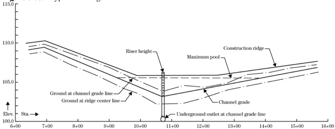
Figure 8-55: Typical Underground Outlet Terrace Profile View
