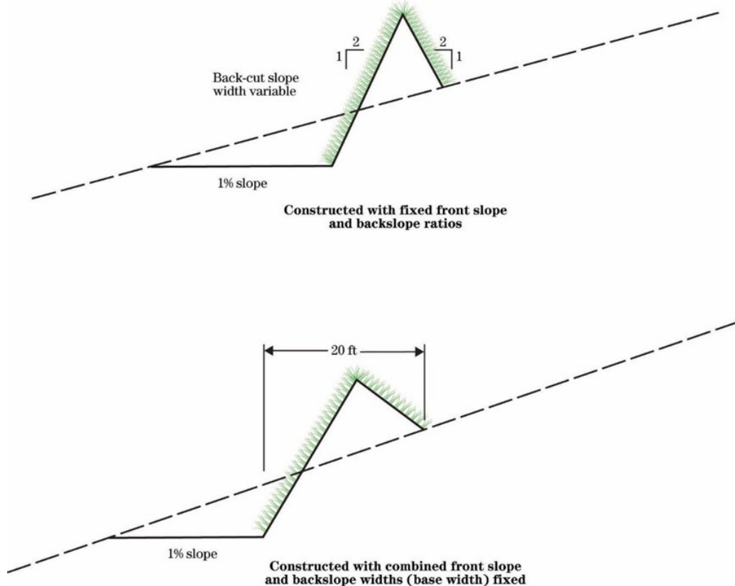
Figure 8-22: Narrow-Base Terrace Cross Section Examples
