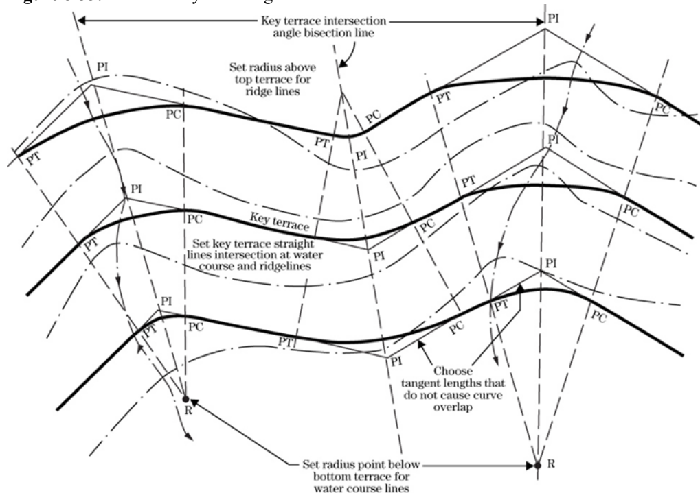
Figure 8-33: Parallel Layout Using Concentric Curve Radius Points
