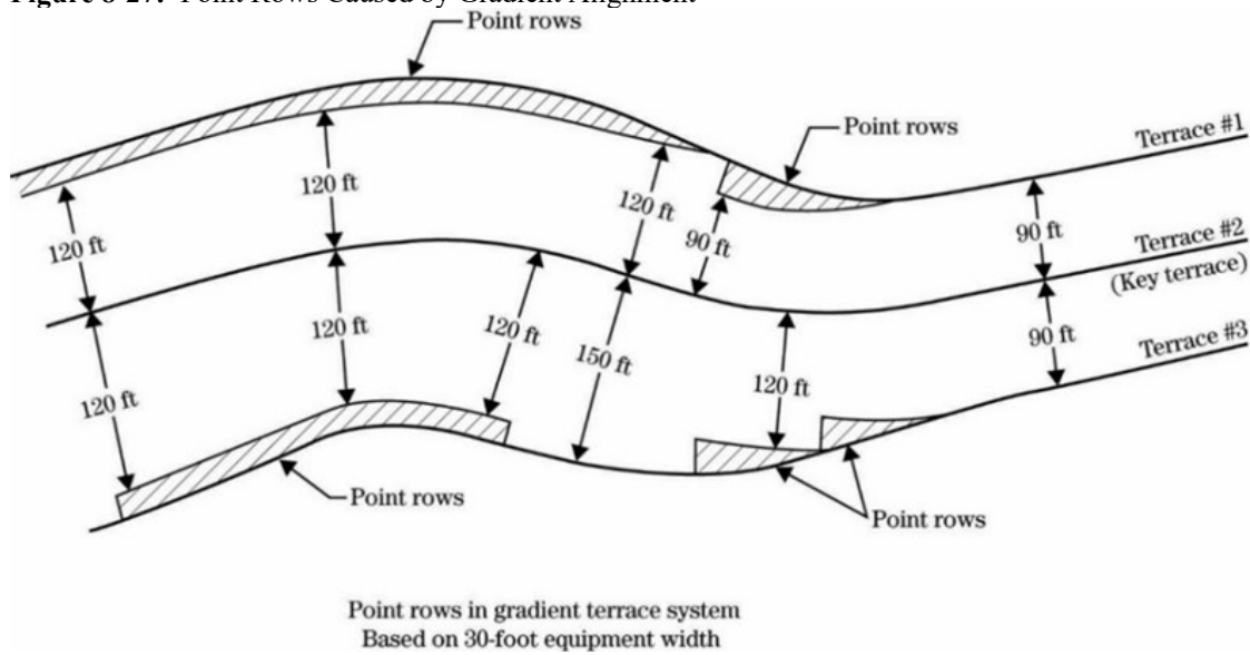
Figure 8-27: Point Rows Caused by Gradient Alignment
