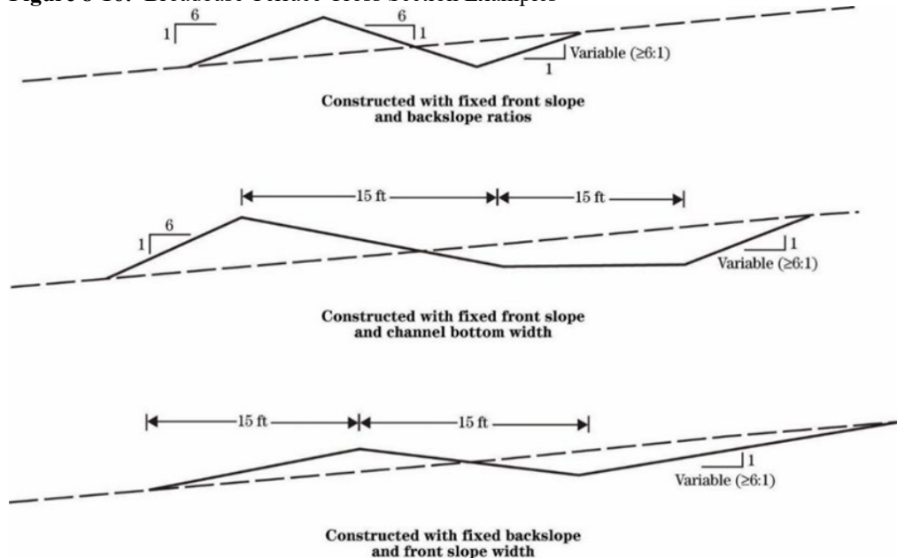
Figure 8-16: Broadbase Terrace Cross Section Examples
