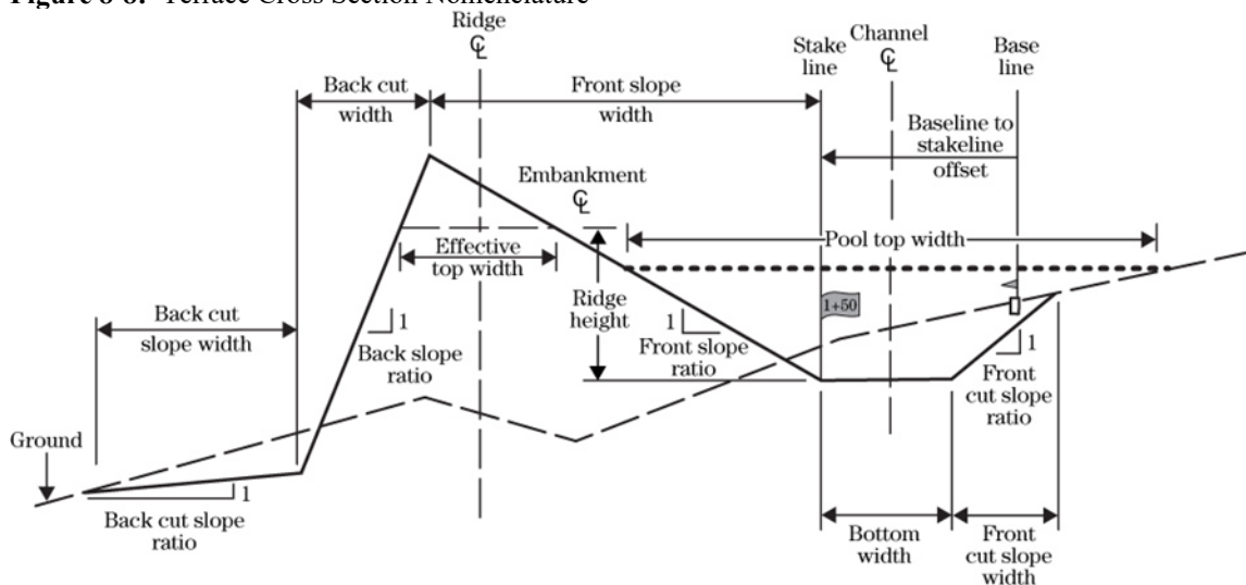
Figure 8-8: Terrace Cross Section Nomenclature
