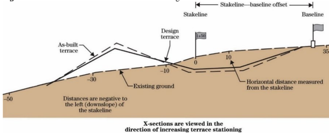
Figure 8-13: Cross Section Measurement and Labeling Conventions
