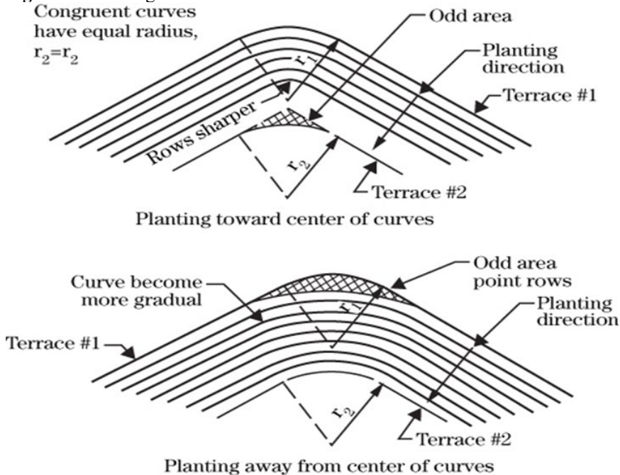
Figure 8-32: Congruent Curves
