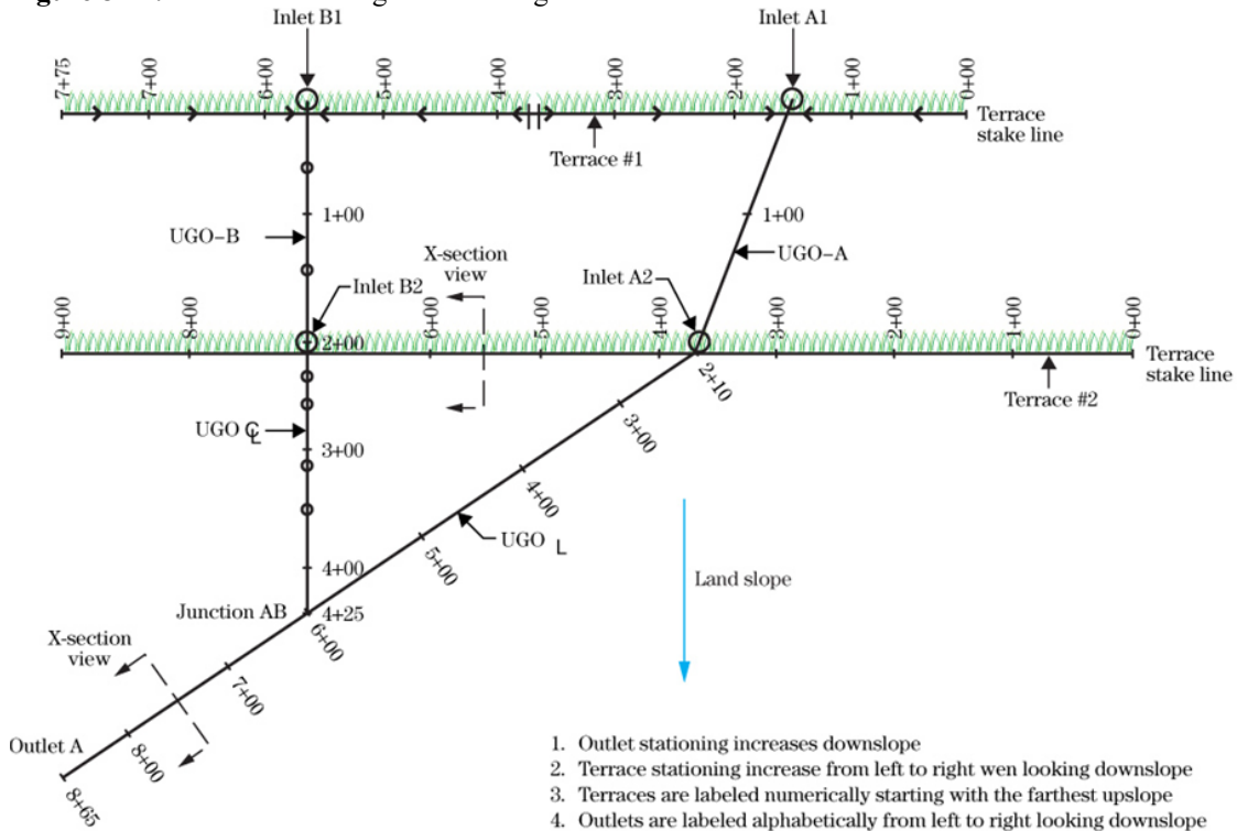
Figure 8-14: Profile Stationing and Labeling Conventions
