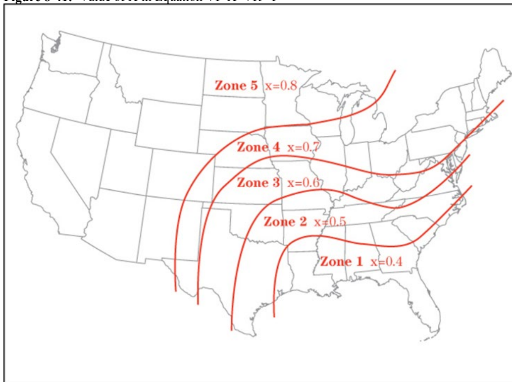
Figure 8-41: Value of X in Equation VI=X \cdot VR+Y
