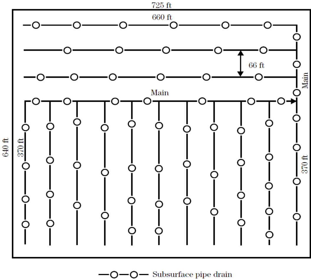
Figure 14-46: Subsurface Drainage System
