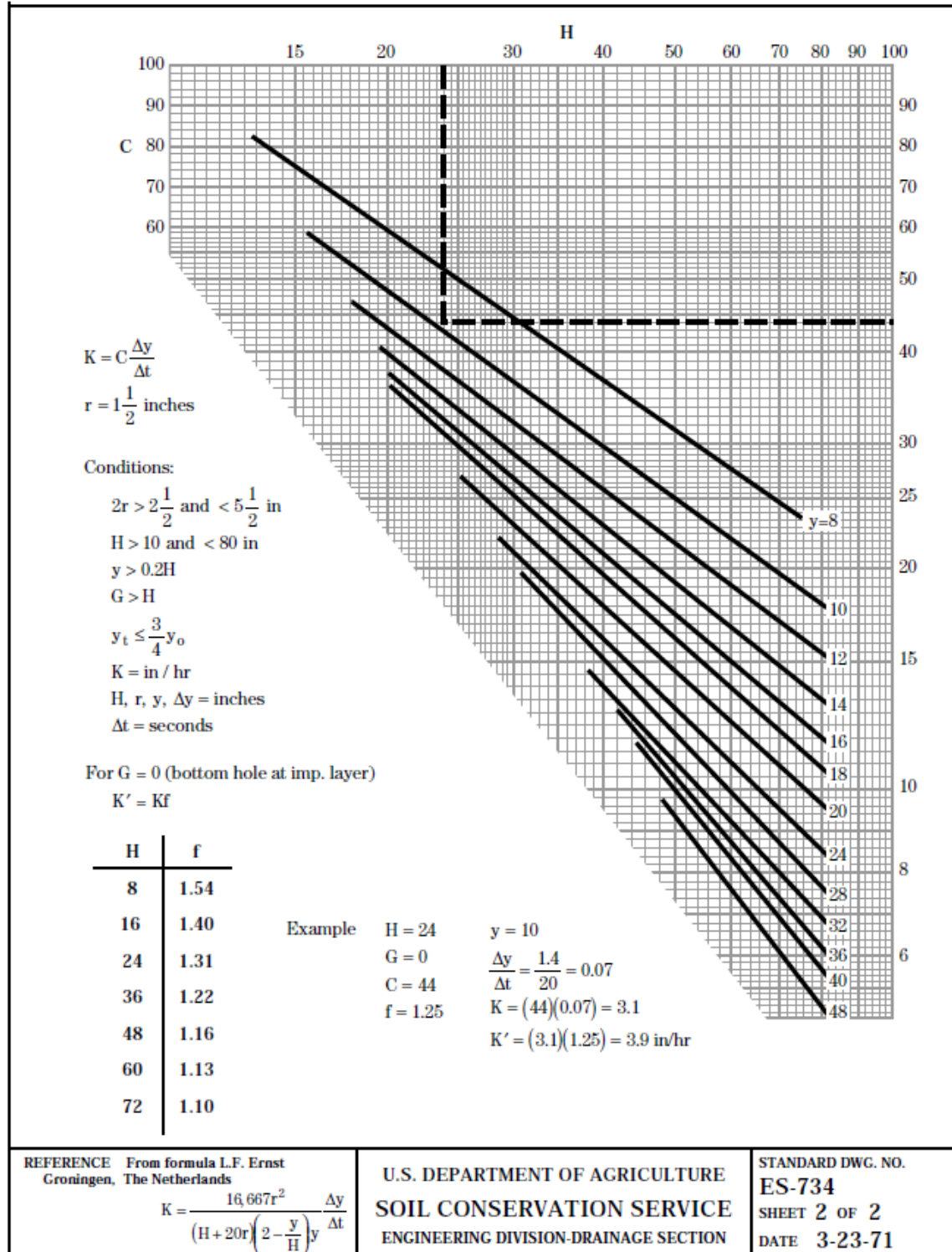
Figure 14D-3. Hydraulic Conductivity—Auger-hole Method Using the Ernst Formula – continued
