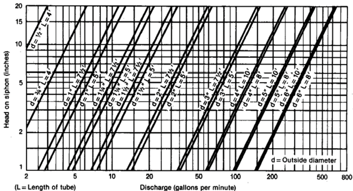
Figure 15-6: Discharge of Aluminum Siphon Tubes at Various Heads
