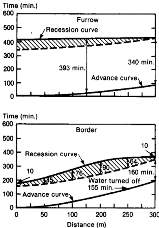
Figure 15-14: Sample Advance and Recession Curves (1)
