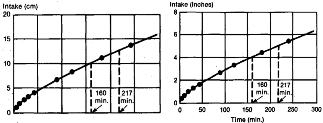
Figure 15-17: Sample Intake Curves
