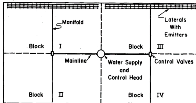
Figure 15-3: Typical Two-station, Split-flow Layout for a Microirrigation System with Blocks I and III, or II and IV Operating Simultaneously
