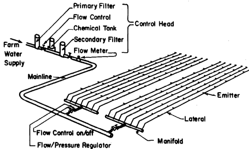
Figure 15-2: Basic Components of a Microirrigation System
