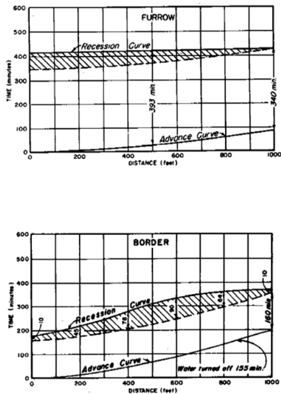
Figure 15-15: Sample Advance and Recession Curves (2)
