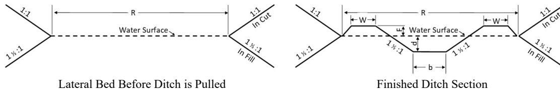
Figure 15-4: Irrigation Ditch Sections with Required Lateral Beds
