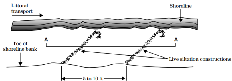
Figure 16-26: Live Siltation
