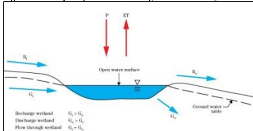
Figure 19-30: Hydrodynamics of Discharge and Flow Through Wetlands
