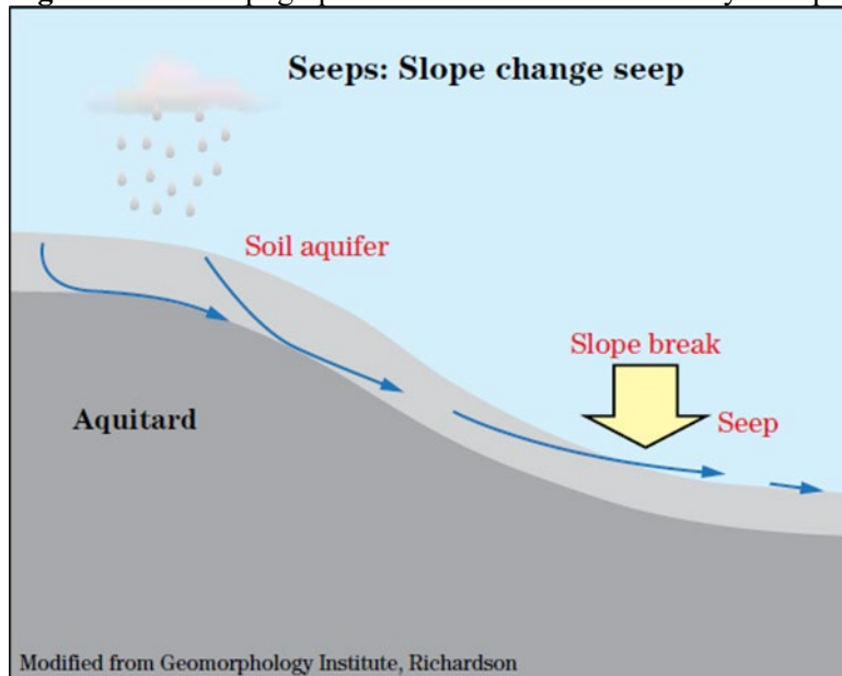
Figure 19-27: Topographic SLOPE Wetland Caused by a Slope Break
