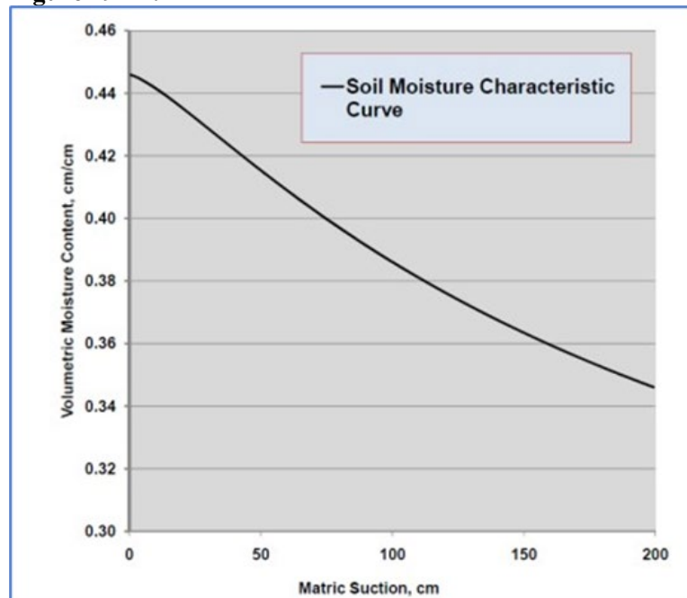
Figure 19-71: Soil Moisture Characteristic Curve
