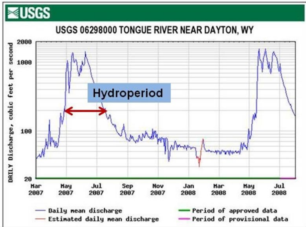
Figure 19-19: Stream Hydrograph Defines RIVERINE Wetland Hydroperiod
