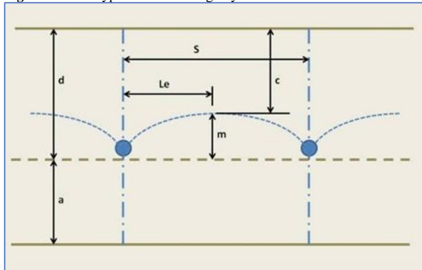
Figure 19-67: Typical Tile Drainage System
