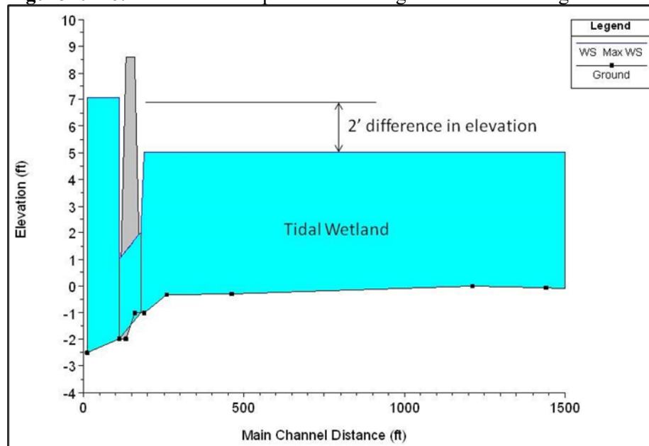
Figure 19-46: HEC-RAS Graphic of Tide Stage and Wetland Stage
