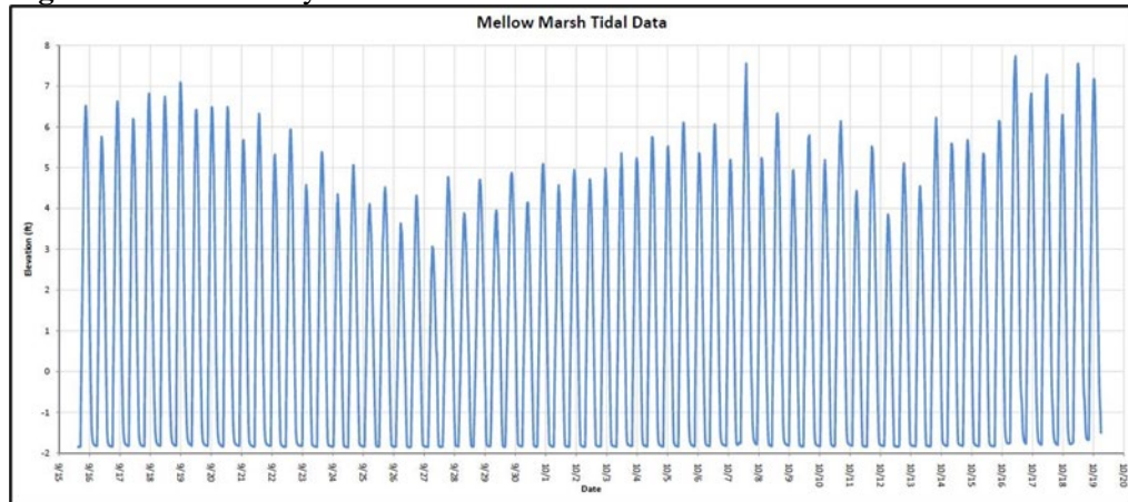
Figure 19-42: Tide Cycles for a One-Month Period
