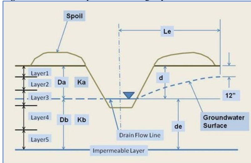
Figure 19-68: Soil Layers in a Drainage System
