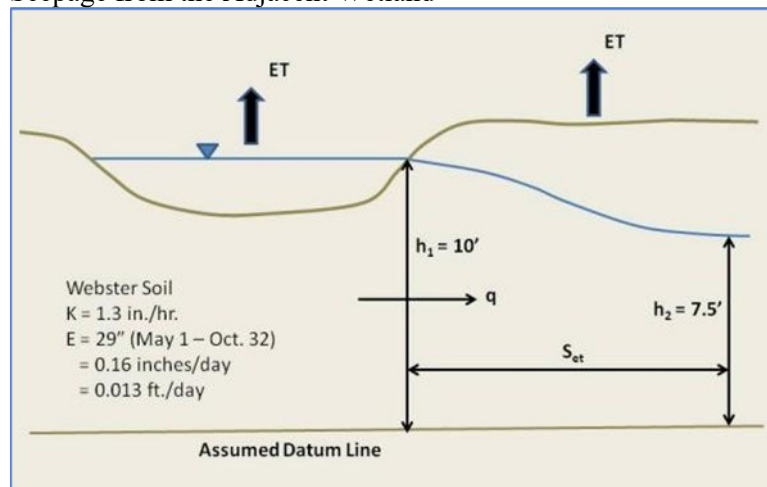
Figure 19-82: Distance over which Water Table Drop due to ET is Replaced by Seepage from the Adjacent Wetland
