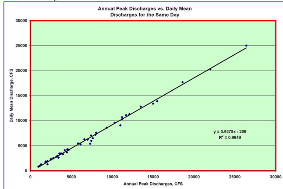
Figure 19-62: Regression Analysis of Annual Peak vs. Corresponding Daily Mean Discharges
