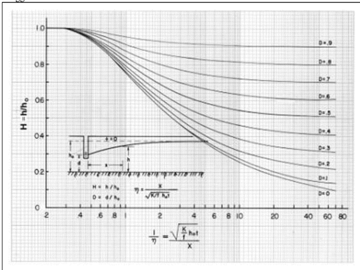
Figure 19-84: Graphical Solutions for Lateral Effect of Drain on an Adjacent Wetland Using the Skaggs Method
