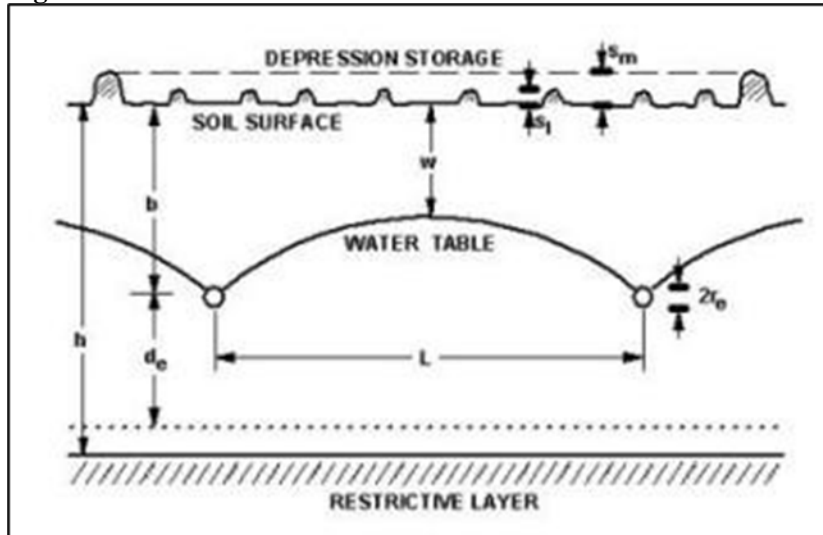
Figure 19-99: Schematic View of DRAINMOD Parameters
