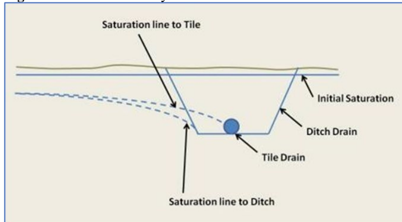
Figure 19-69: Water Entry into Ditch and Tile
