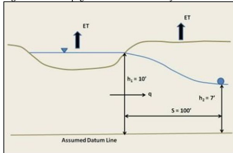
Figure 19-83: Seepage from Wetland with Adjacent Tile Drain
