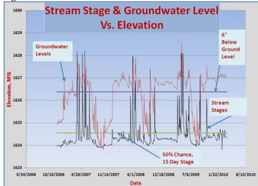
Figure 19-57: Plot of Streamflow and Groundwater Level vs. Time
