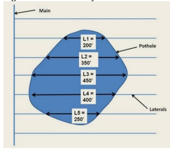
Figure 19-81: Drain Layout for Kirkham's Equation Example
