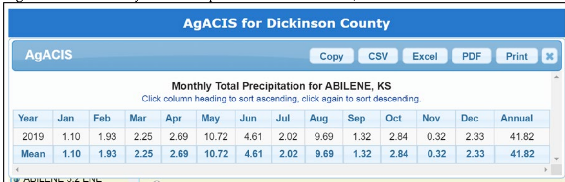
Figure 19-33: Monthly Total Precipitation Data for Abilene, Kansas - 2019
