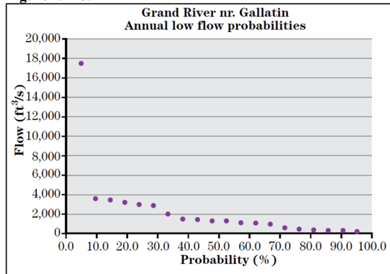
Figure 19-48: Plot of Annual Duration Flows
