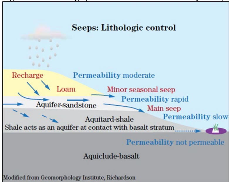
Figure 19-26: Stratigraphic SLOPE Wetland Created by an Aquitard
