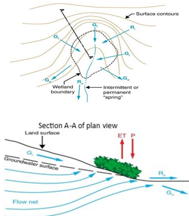
Figure 19-25: Plan View of Topographic SLOPE Wetland in Concave Landscape Position at Stream Headwaters
