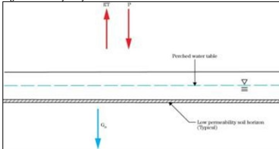
Figure 19-28: Hydrodynamics of MINERAL SOIL FLATS Wetlands
