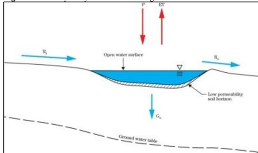
Figure 19-29: Hydrodynamics of Recharge DEPRESSIONAL Wetlands
