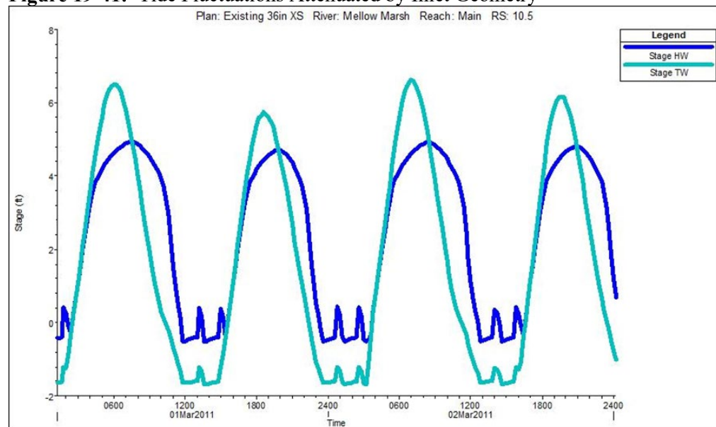
Figure 19-41: Tide Fluctuations Attenuated by Inlet Geometry
