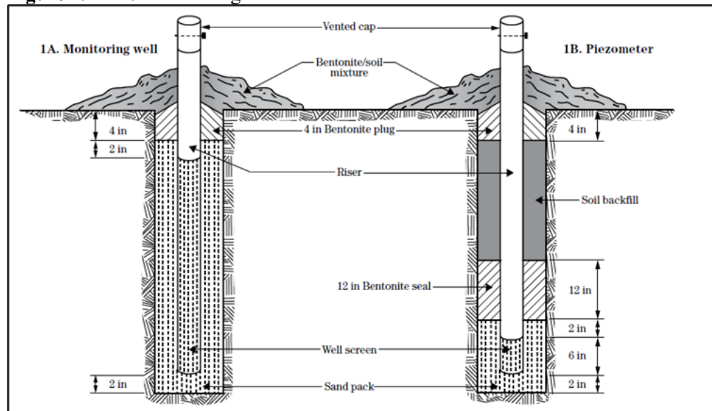
Figure 19-112: Monitoring Well and Piezometer Installation
