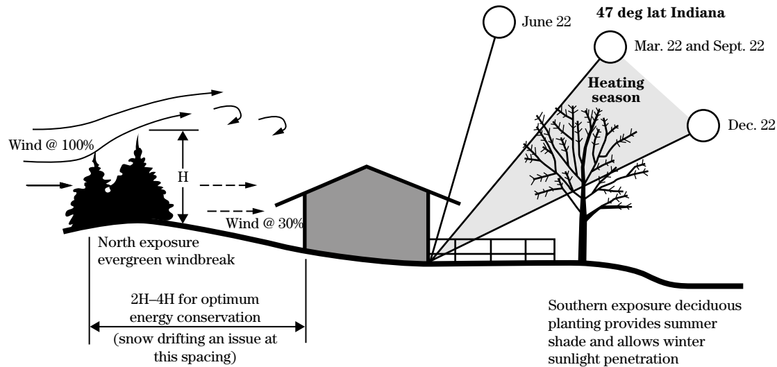
Figure 8-23 Vegetation modifies temperature in various ways.
