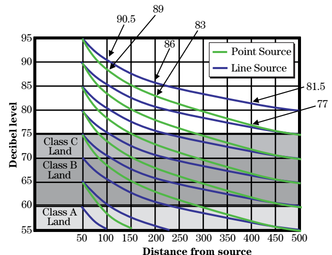
Figure 8–30 Noise reduction by distance from source
