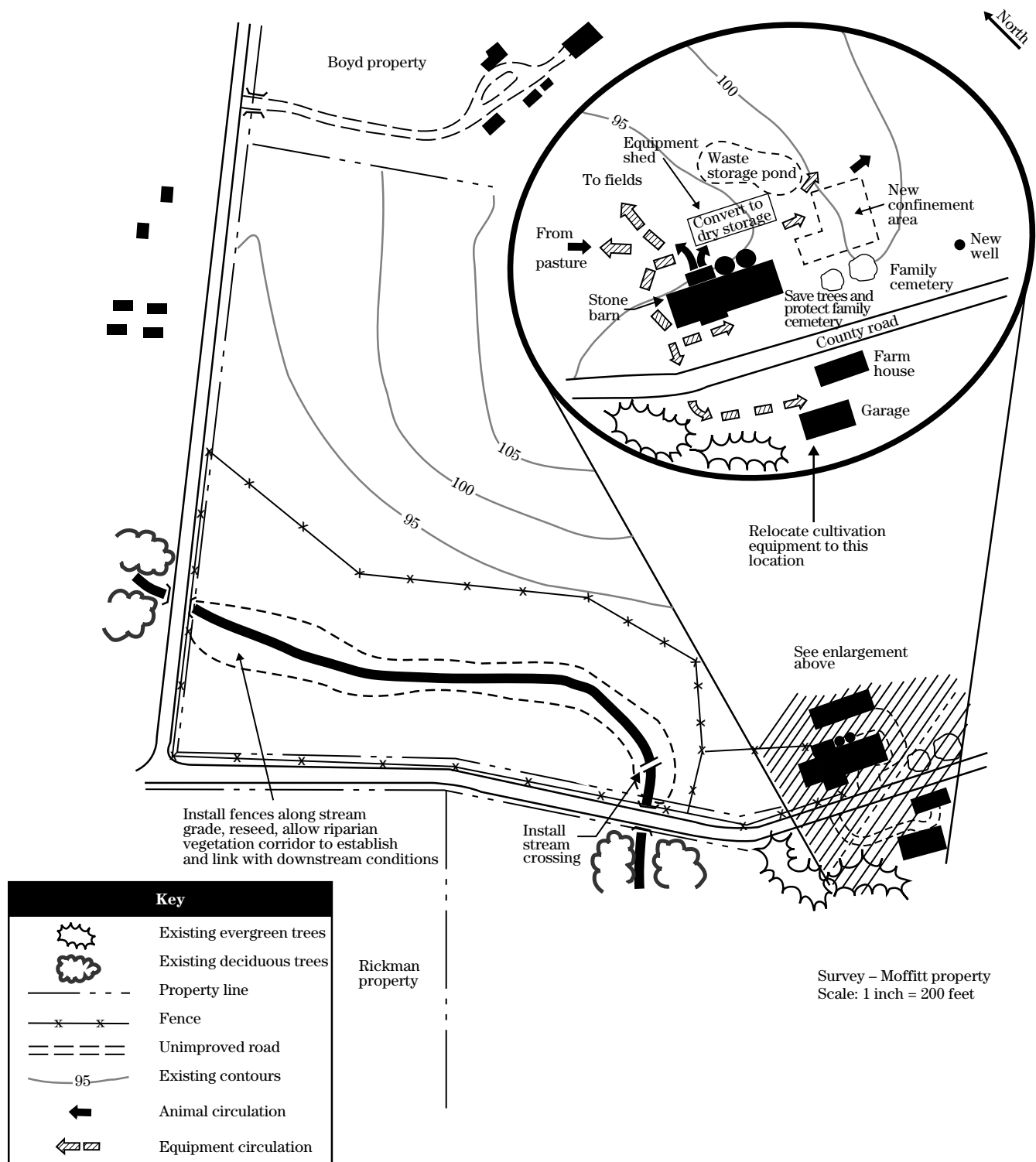
Figure 8-3 Concept plan
