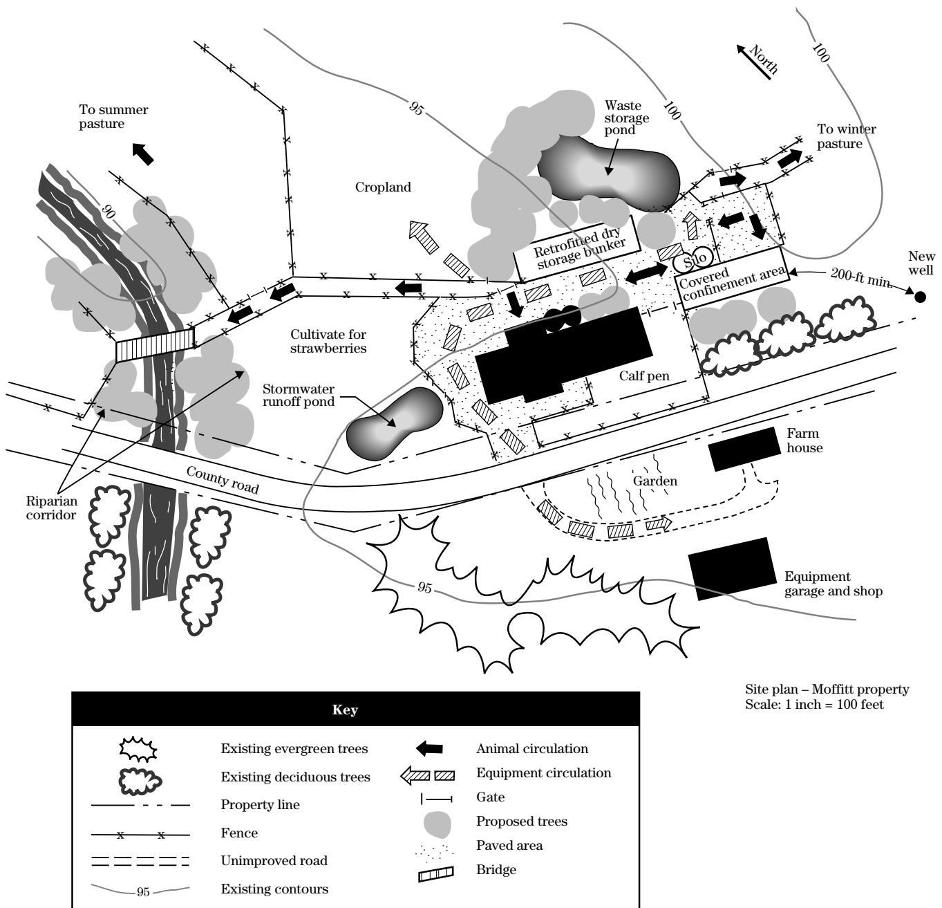
Figure 8-4 Site plan
