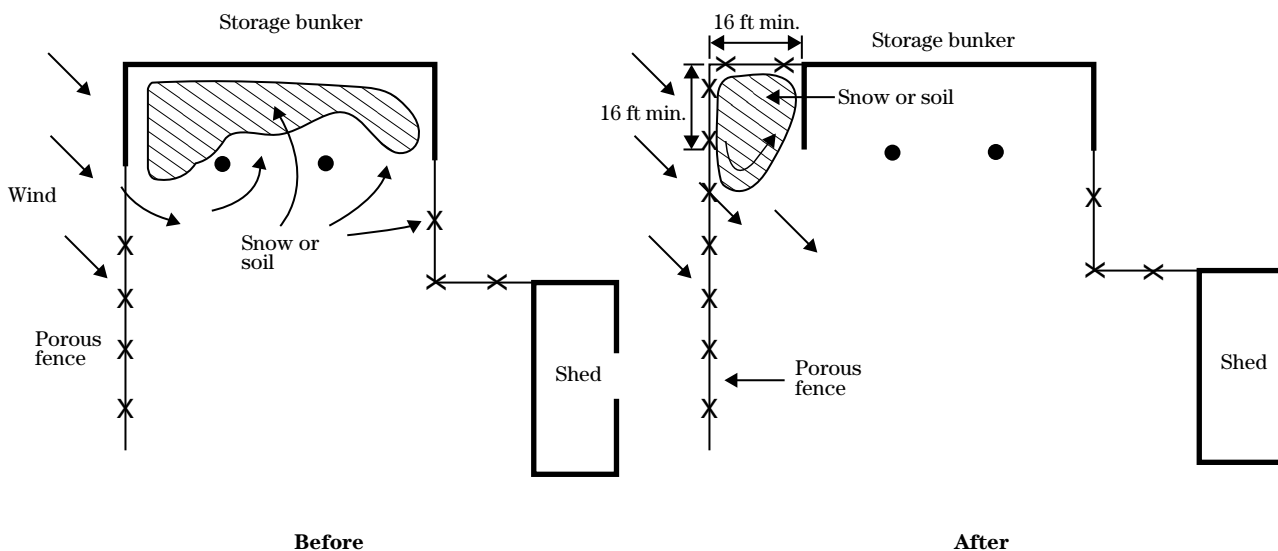
Figure 8-27 Fences affect snow and soil deposition around buildings.
