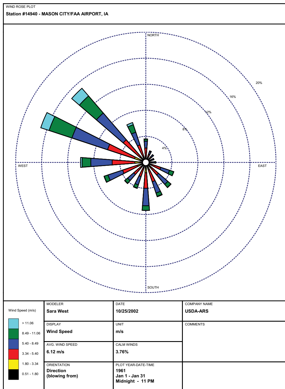
Figure 8–28 Wind rose diagrams can be used to determine prevailing wind directions. This wind rose diagram is for January from Mason City, IA.
