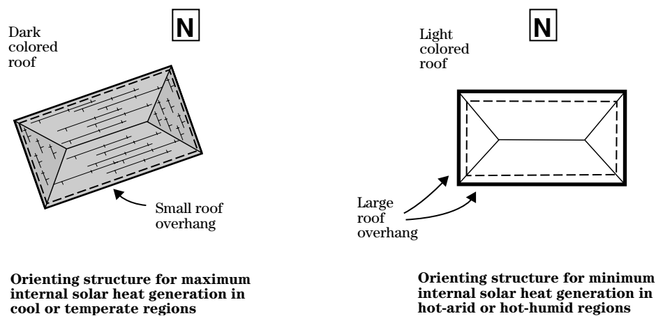
Figure 8-24 Orientation can influence the amount of internal sun-generated heat within buildings.
