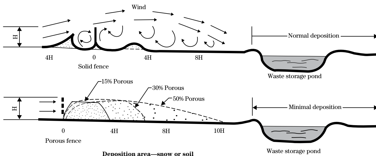
Figure 8–25 Fence porosity affects snow deposition
