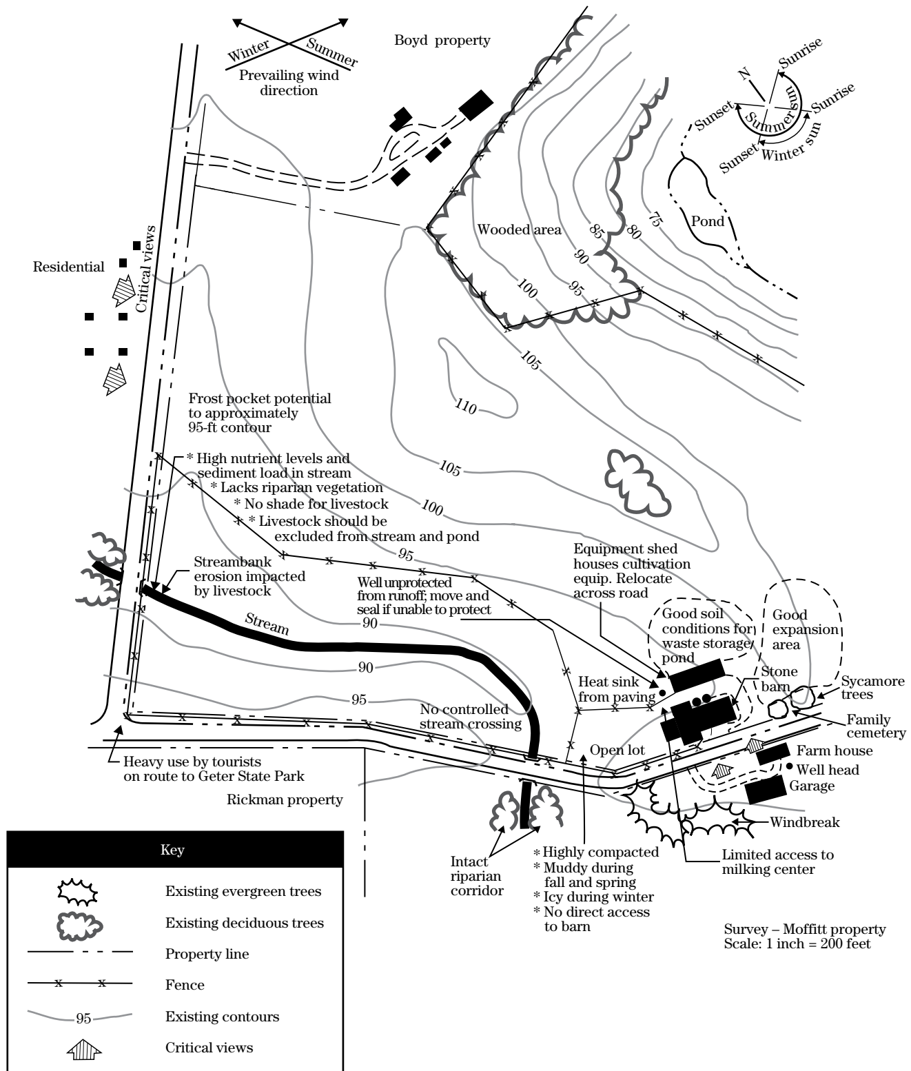
Figure 8-2 Site analysis diagram
