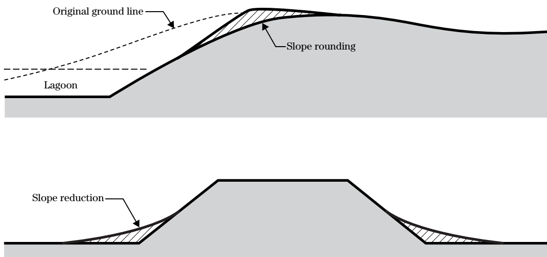
Figure 8-7 Slope rounding and reduction help to blend landforms onto the landscape.
