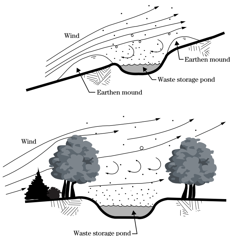
Figure 8–22 Topography, structures, and vegetation can uplift winds to disperse odor.
