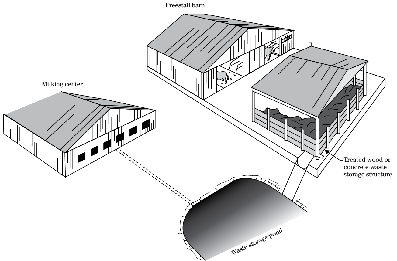
Figure 9-8 Storage facilities
