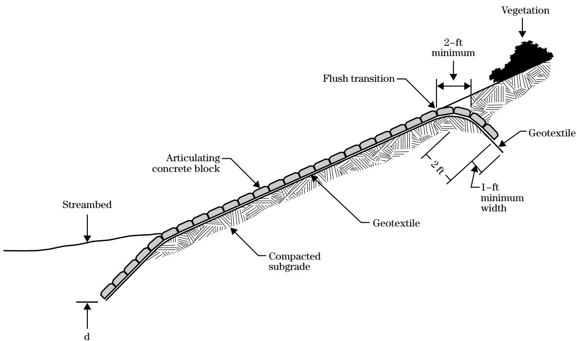
Figure TS14L-2 Armoring the toe and lower slope cross section
