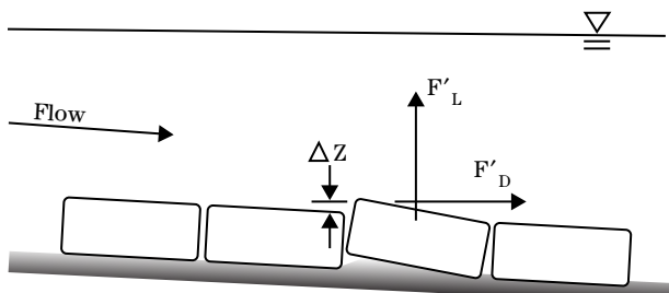
Figure TS14L-14 Forces on a protruding block (Figure courtesy of HCFCD)
