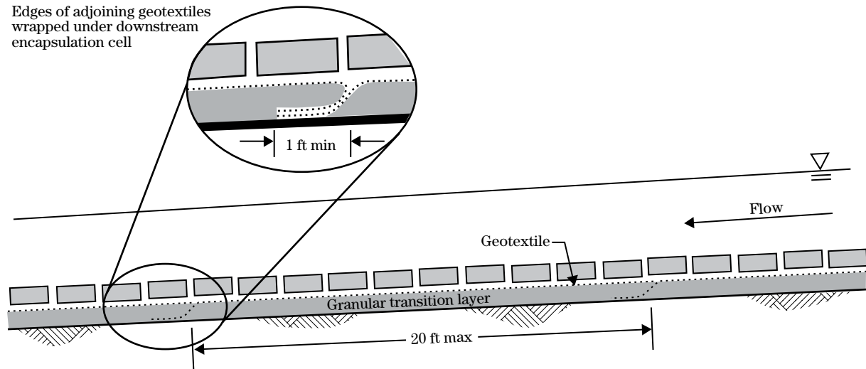
Figure TS14L-17 Granular filter encapsulation by a geotextile ( Figure courtesy of HCFC )
