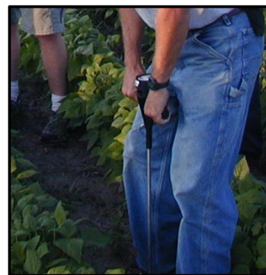
Figure 8: Applying slow, steady pressure when pushing penetrometer into soil
