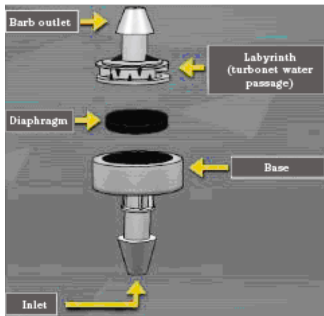
Figure 7–60 Schematic of a pressure compensated, turbulent flow button emitter (courtesy Netafim USA)
