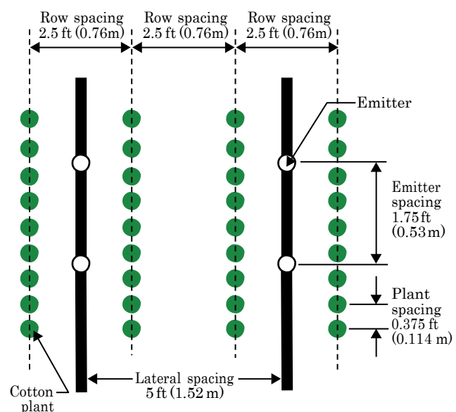
Figure 7-117 Emitter/lateral/plant/row layout
