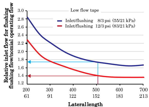
Figure 7-89 Relative flow requirements during flushing for low flow tape. ID = 0.625 in (15.9 mm), Q=0.22 gal/min/100 ft at 8 and 12 psi (1.64 L/h/m at 55 and 83 kPa) inlet pressure (adapted from Burt and Styles 1994)
