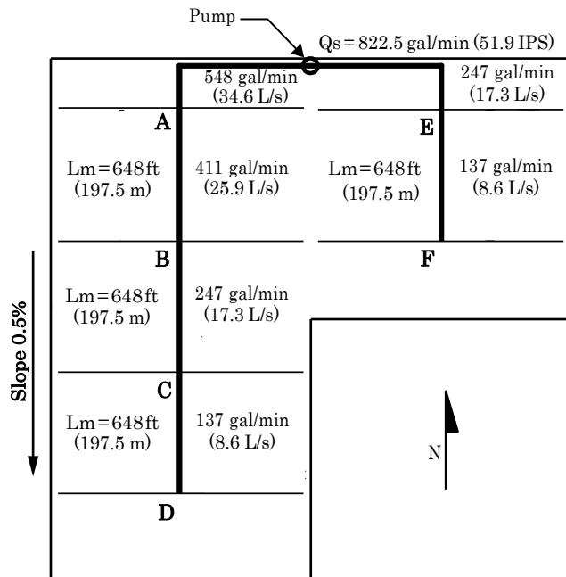
Figure 7–98 Orchard layout showing pump, mainline, and submains
