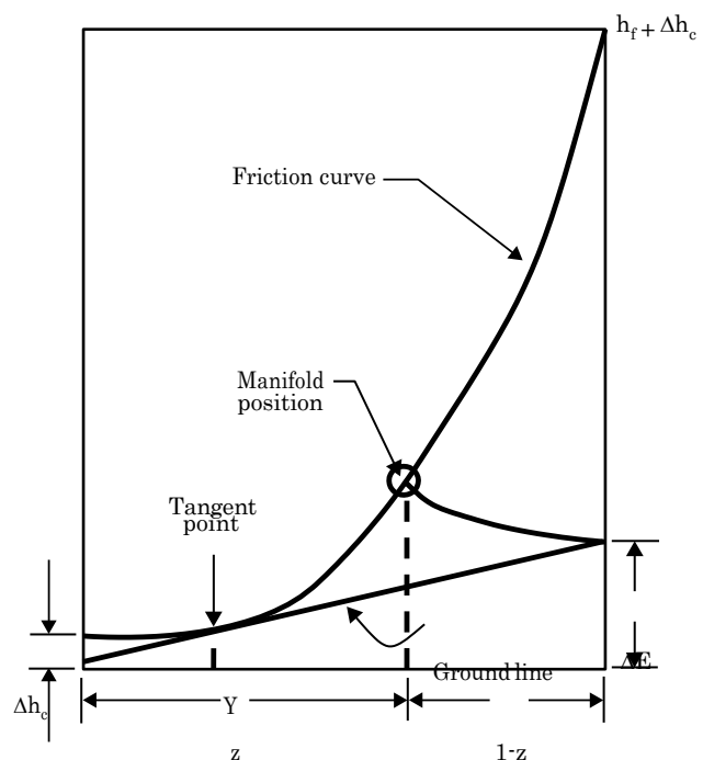
Figure 7-93 Sketch showing relationship between manifold position and lateral hydraulics for a paired lateral
