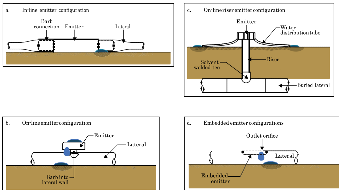
Figure 7-83 Lateral connectors
