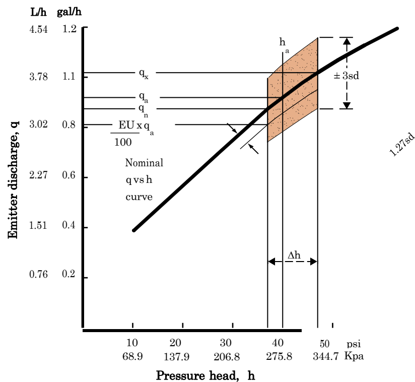
Figure 7–88 Combined effect of pressure head and manufacturing variations on discharges of individual emitters
