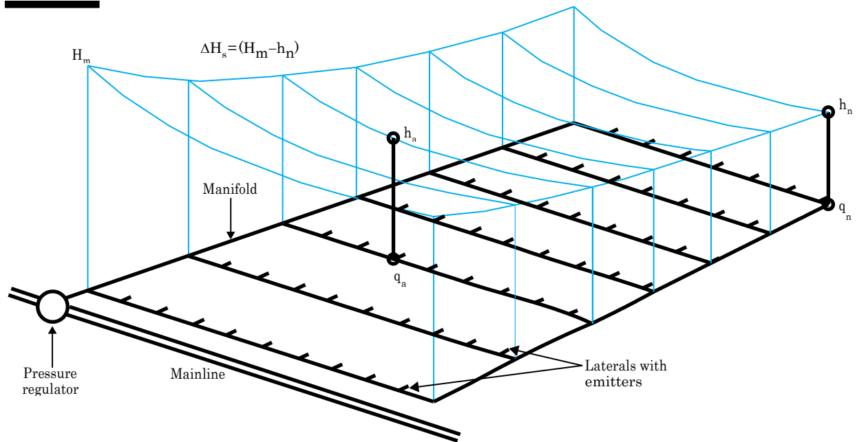
Figure 7–87 Distribution of a pressure head in a subunit
