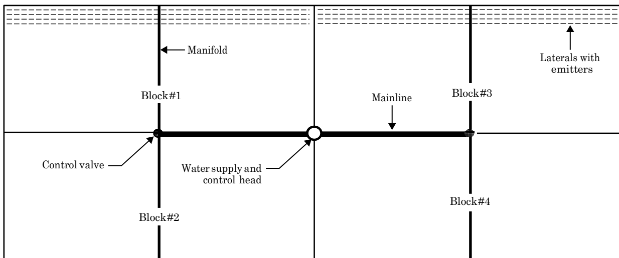
Figure 7–86 Typical two-station, split-flow layout for drip irrigation system with blocks I and III, or II and IV, operating simultaneously
