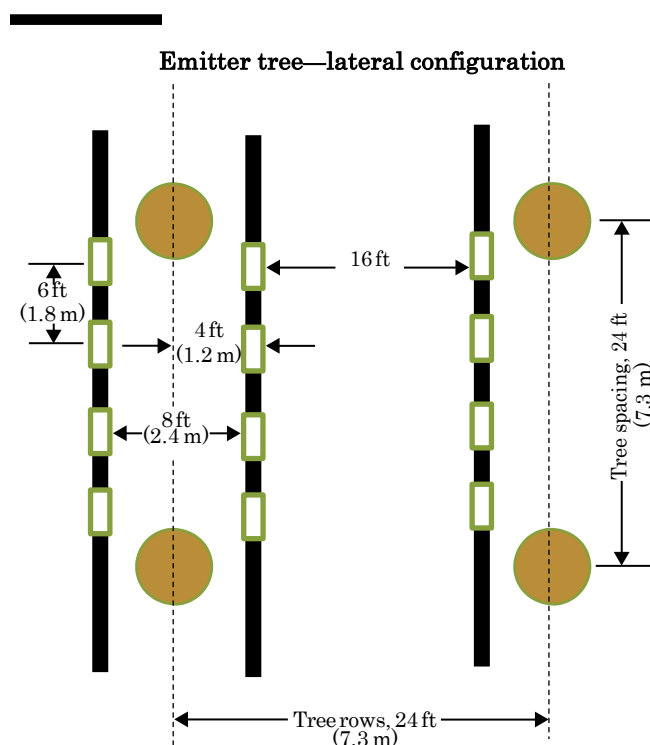
Figure 7-107 The emitter/lateral/tree row layout
