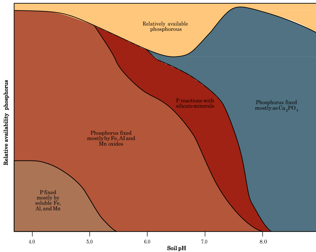
Figure 7–16 Relative availability of added phosphorus in soil as affected by soil pH (adapted from Buckman and Brady 1966)
