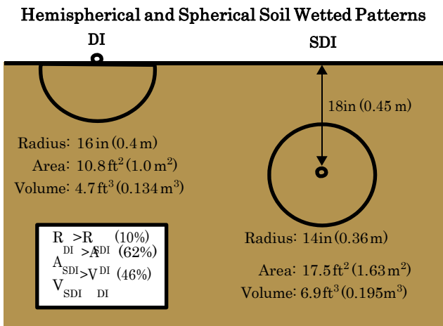
Figure 7–71 Simulated soil wetted patterns created in a dry Panoche clay loam soil
