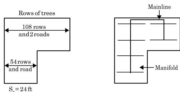
Figure 7-101 Manifold layout
