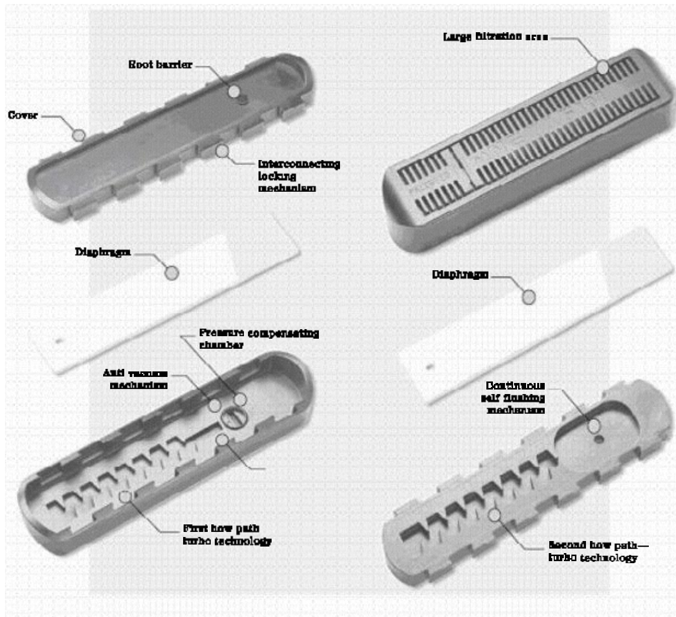
Figure 7–76 Components and features of a PC–CNL emitter (courtesy of Netafim Irrigation)
