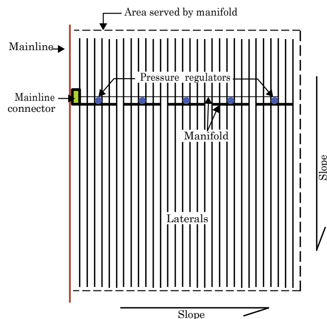
Figure 7–50 Manifold layout showing inlet connection uphill from center and showing pressure regulated manifolds
