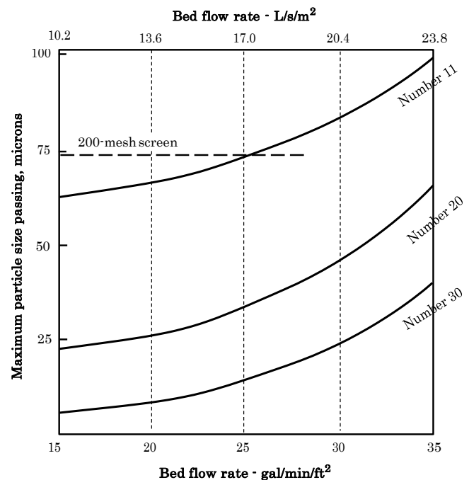
Figure 7–25 Effect of flow rate on the maximum particle size passing through a typical free-flow sand filter with media of various sizes
