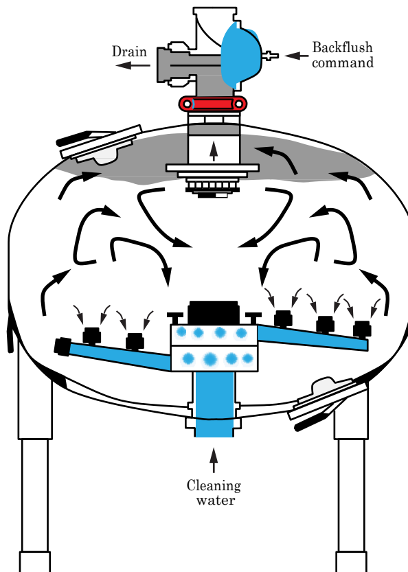
(b) Backflushing mode
