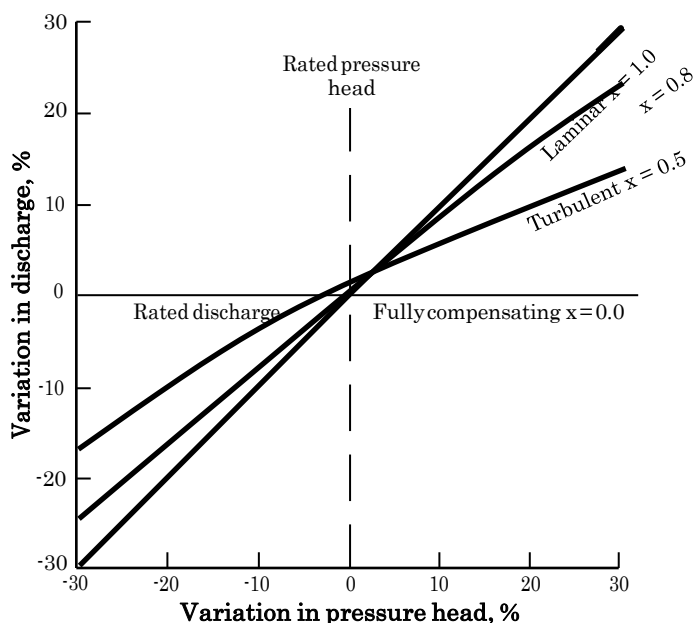
Figure 7-79 Relationship between percentage variations in discharge as affected by the percentage variation in pressure head for various emitters with different discharge exponents (Keller and Karmeli 1974)
