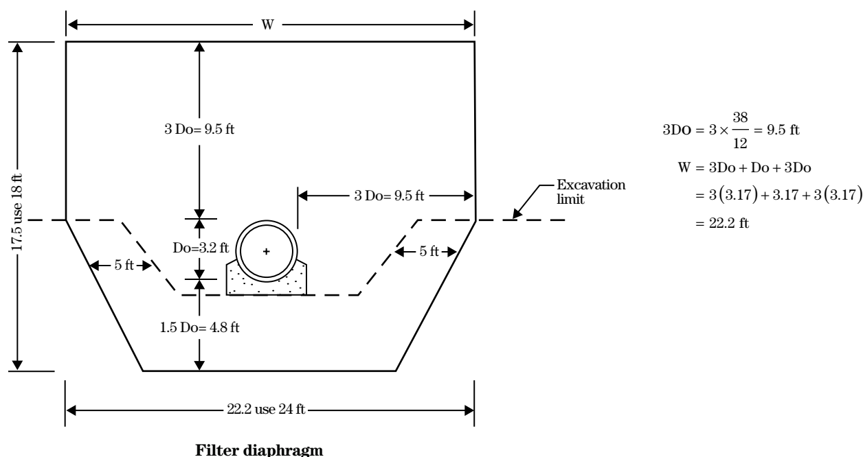
Figure 45C-2 Filter diaphragm for example 1
