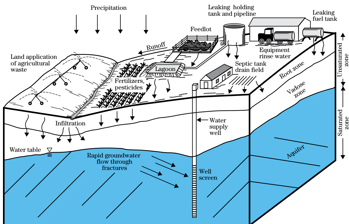
Figure 7–1 Agricultural sources of potential groundwater contamination
