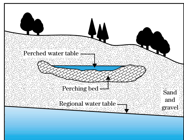
Figure 7-8 Perched aquifer
