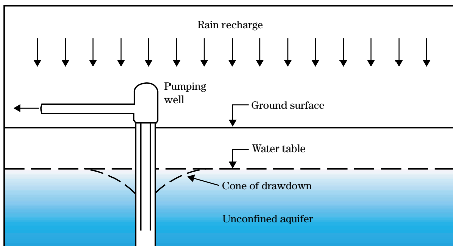
Figure 7-5 Unconfined aquifer (AIPG 1984)
