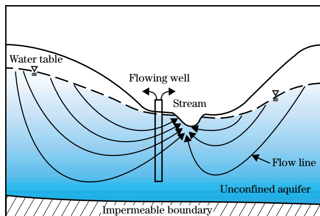
Figure 7-7 Cross section through stream valley showing groundwater flow lines and flowing (artesian) well from unconfined aquifer (Fetter 1980)
