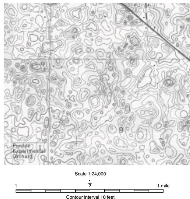
Figure 7–10 Karst topography
