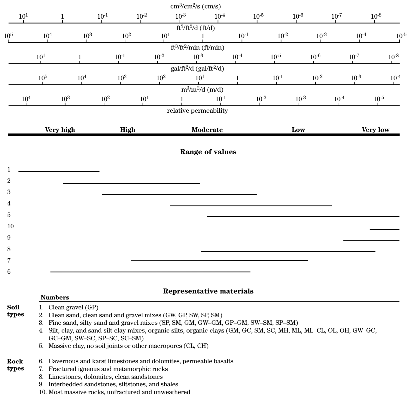
Figure 7-11 Permeability of various geologic materials (from Freeze and Cherry 1979)
