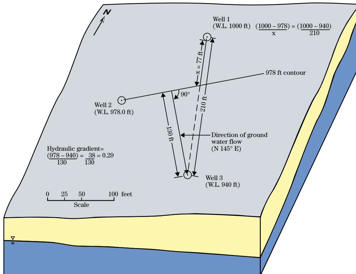
Figure 7A-1 Determining direction of groundwater flow and hydraulic gradient (from Heath 1983)
