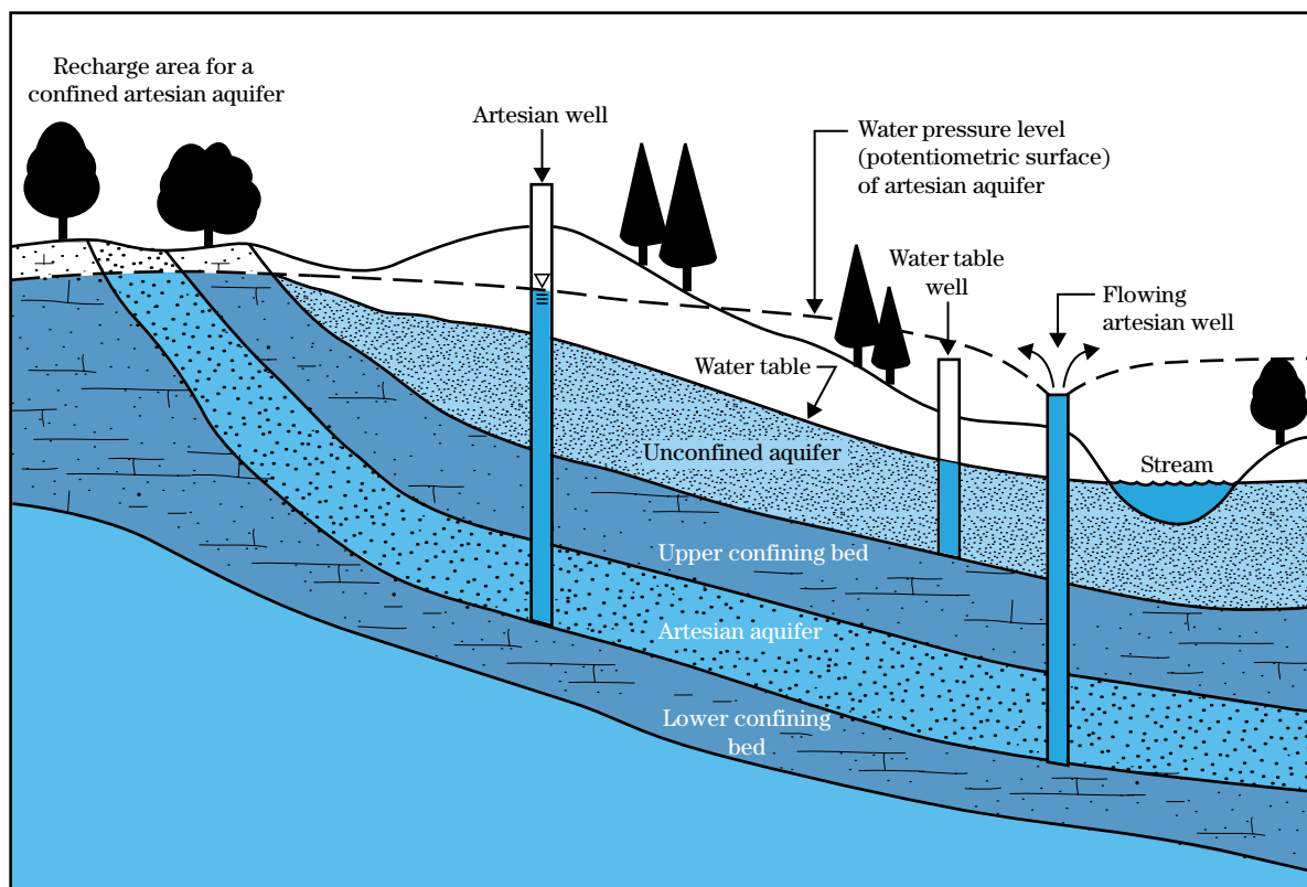
Figure 7-4 Aquifers (AIPG 1984)
