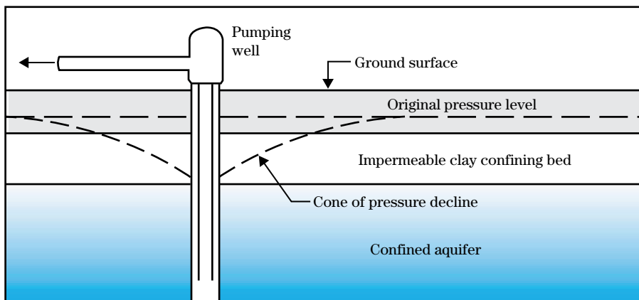
Figure 7-6 Confined (artesian) aquifer (AIPG 1984)
