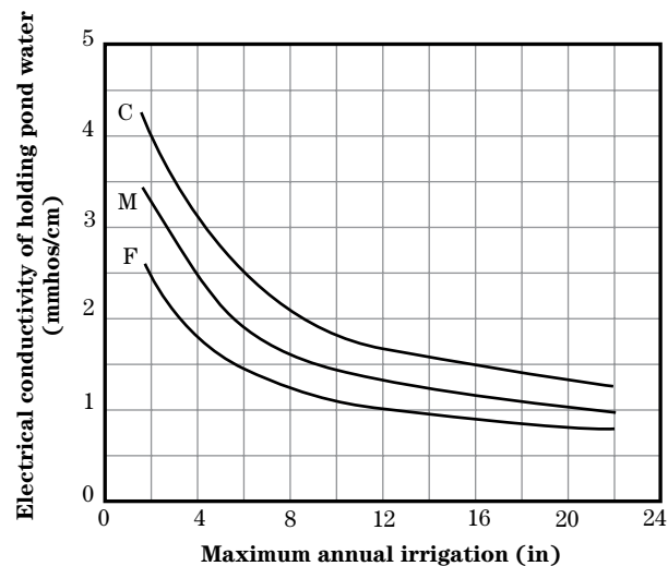
Figure 11-8 Maximum annual amount of undiluted waste storage pond water that can be added to a coarse (C), medium (M), or fine-textured (F) soil
