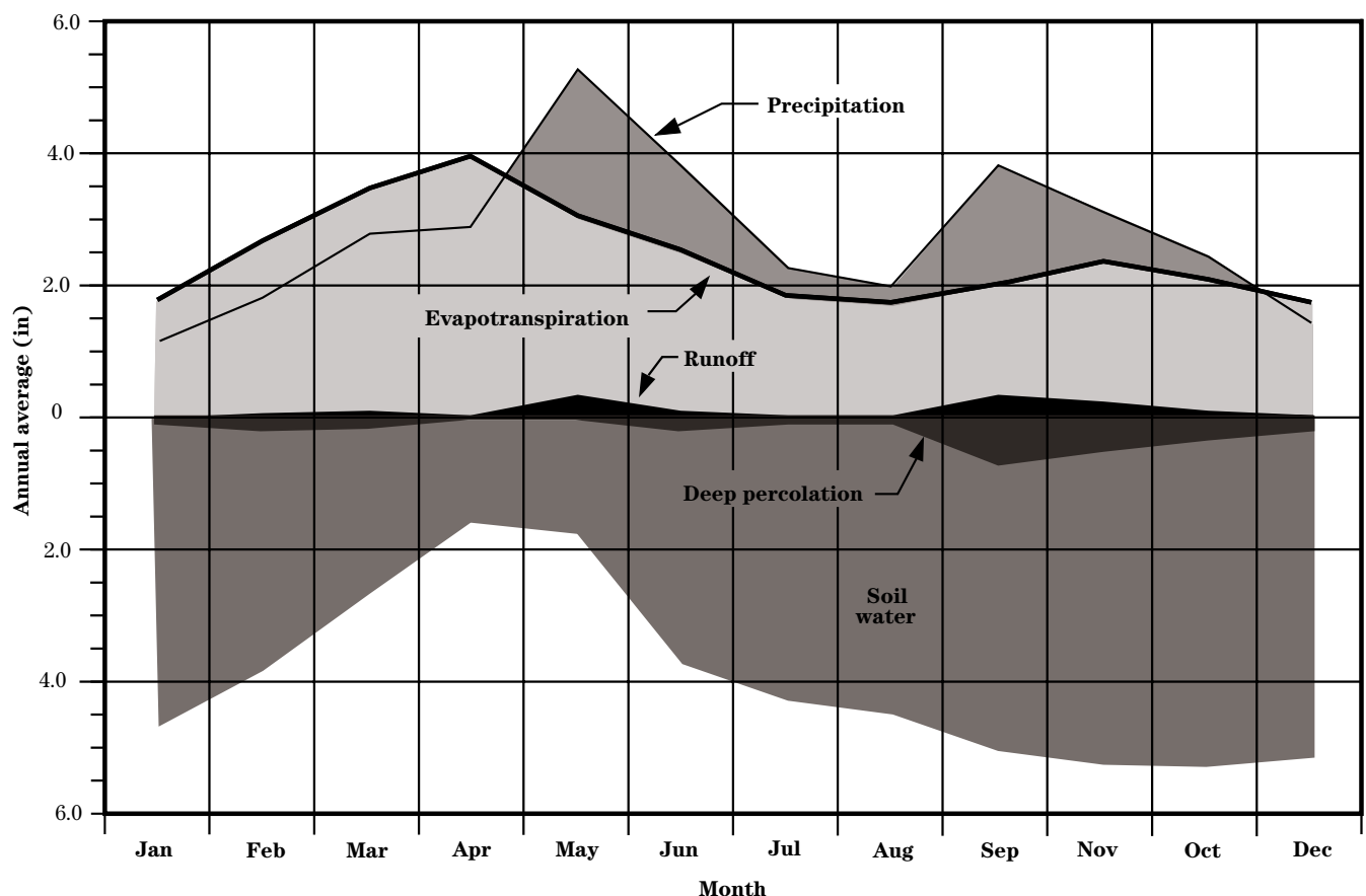
Figure 11-10 Example of a water budget for winter wheat
