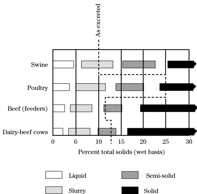
Figure 11–1 Relative handling characteristics of different types of manure and percent TS (ASAE 1990)
