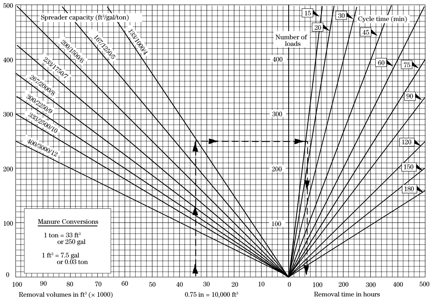
Figure 11-4 Removal time for various cycle times and spreader capacities
