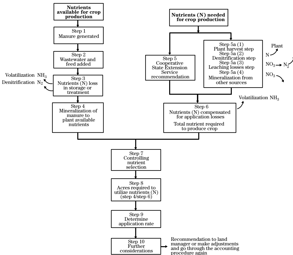
Figure 11-11 Nitrogen transformation in the accounting procedure
