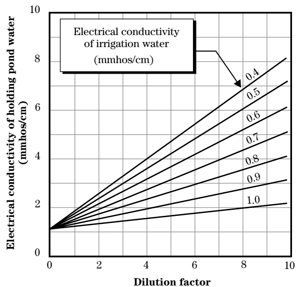
Figure 11-6 Waste storage pond dilution factors for resulting low salinity on medium-textured soils
