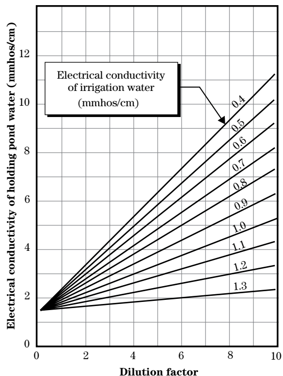
Figure 11-5 Waste storage pond dilution factors for resulting low salinity on coarse-textured soils
