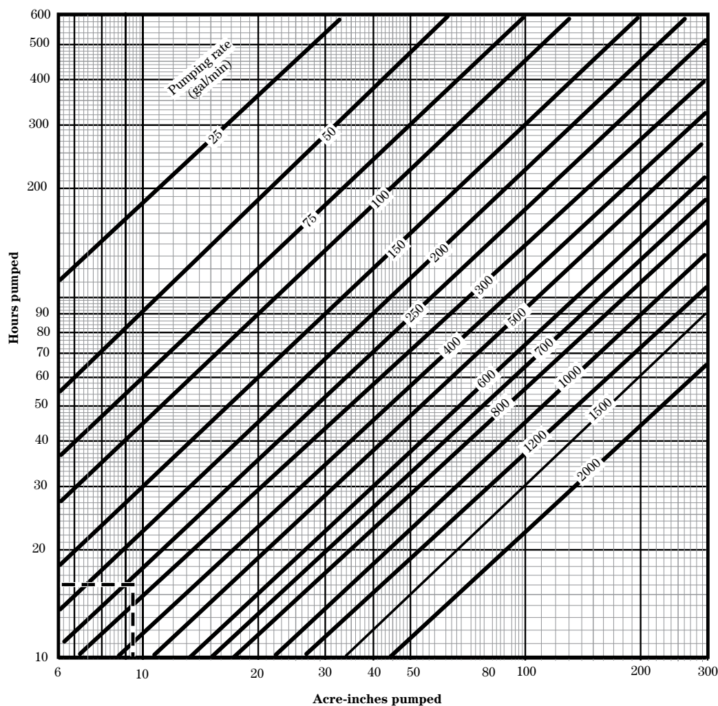
Figure 11-3 Acre inches pumped in given time at various pumping rate
