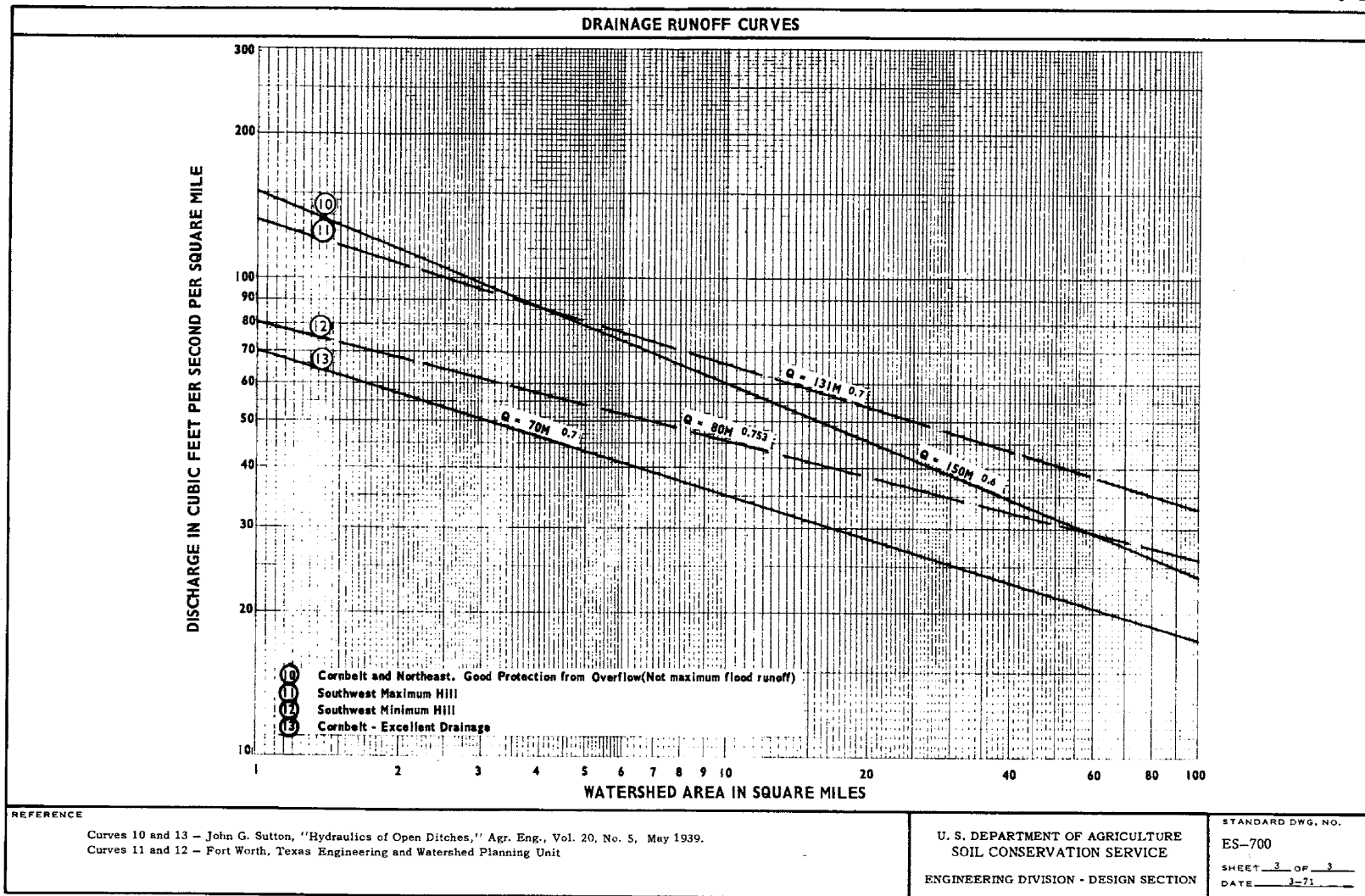
Figure 5-3, Drainage runoff curves
