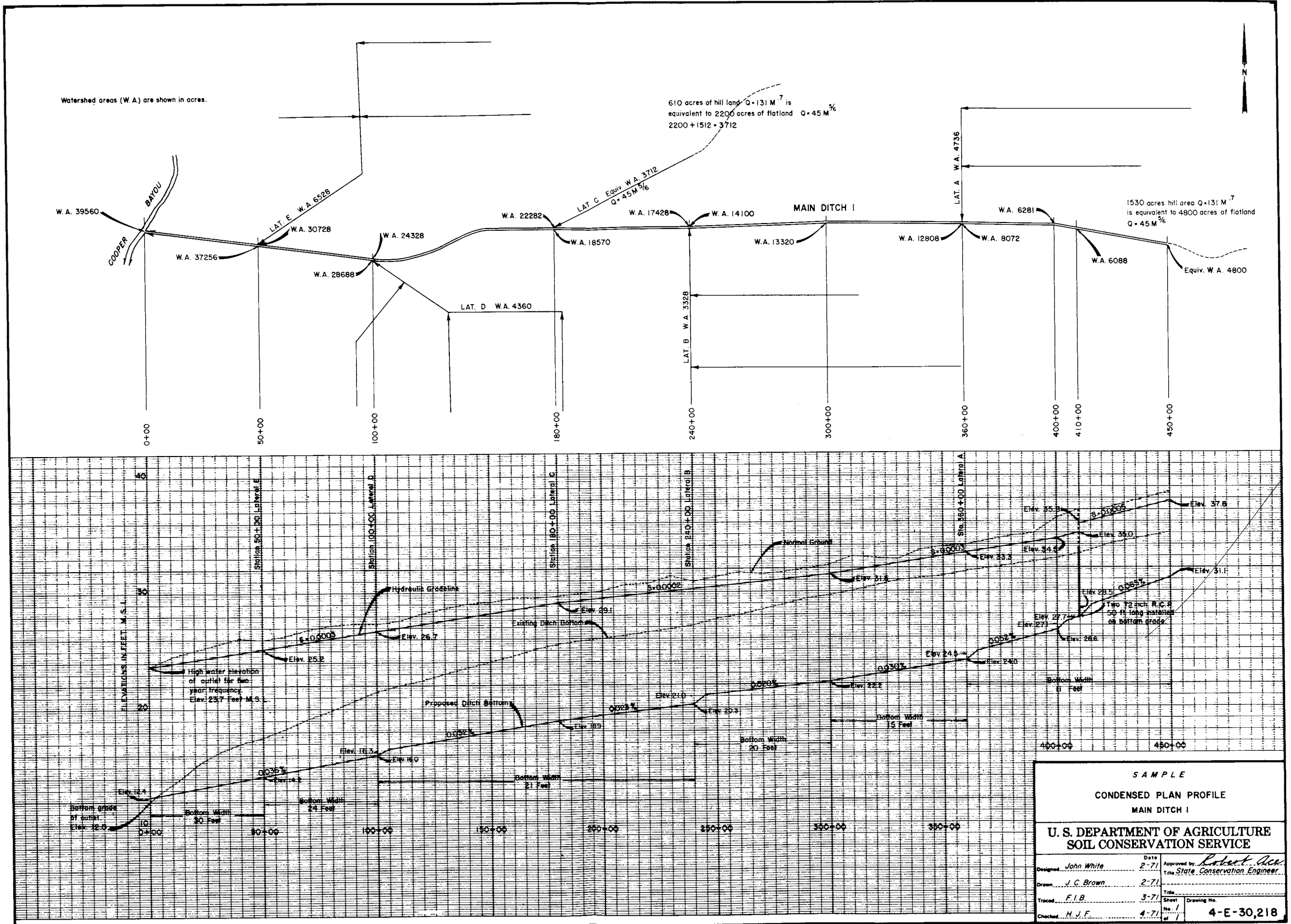
Figure 5-7, Sample--Condensed plan profile
