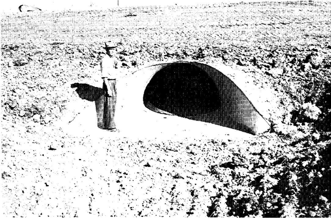
Prefabricated entrance section on pipe drop
